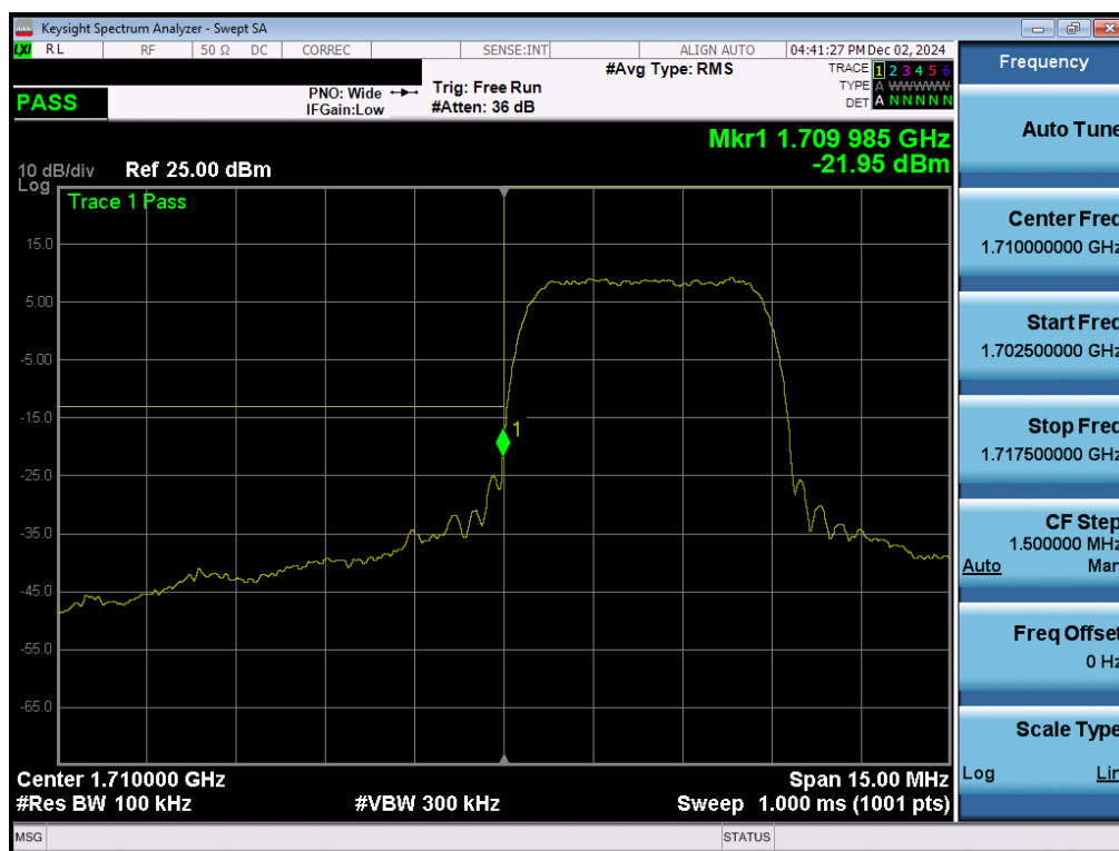
Plot 7-196. Lower Band Edge Plot (WCDMA AWS – Ch. 1312 – Ant 1)
