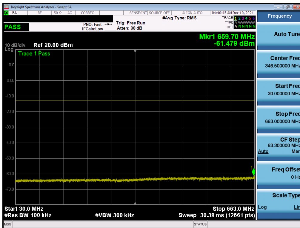
Plot 7-145. Conducted Spurious Plot (NR Band n71 - 20.0MHz - 1 RB - Mid Channel - Ant 2)
