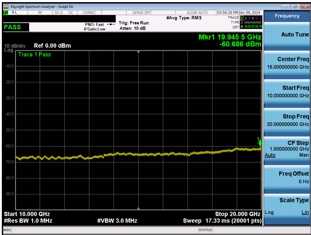
Plot 7-163. Conducted Spurious Plot (NR Band n66 - 40.0MHz - 1 RB - High Channel - Ant 1)
