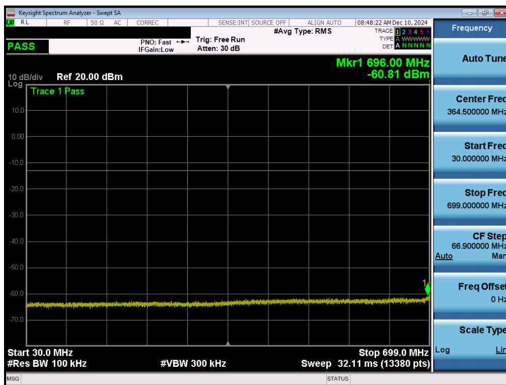
Plot 7-129. Conducted Spurious Plot (NR Band n12 - 15.0MHz - 1 RB - Mid Channel - Ant 5)
