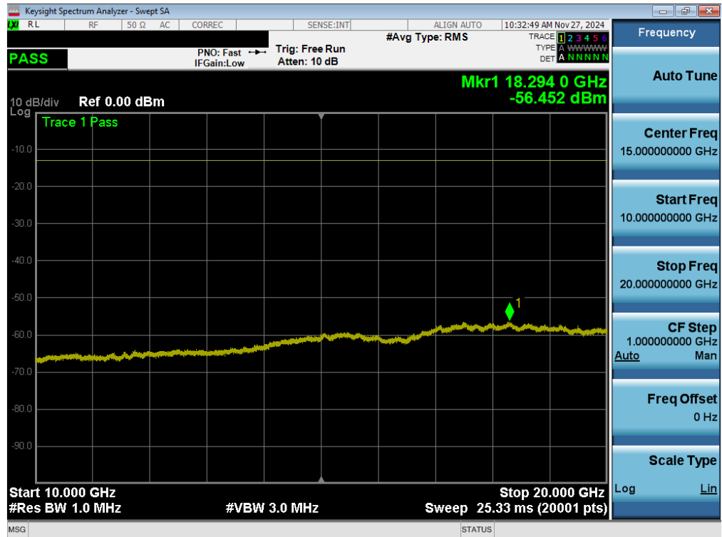
Plot 7-160. Conducted Spurious Plot (LTE Band 66/4 - 20MHz QPSK - 1 RB - Mid Channel – Ant 1)
