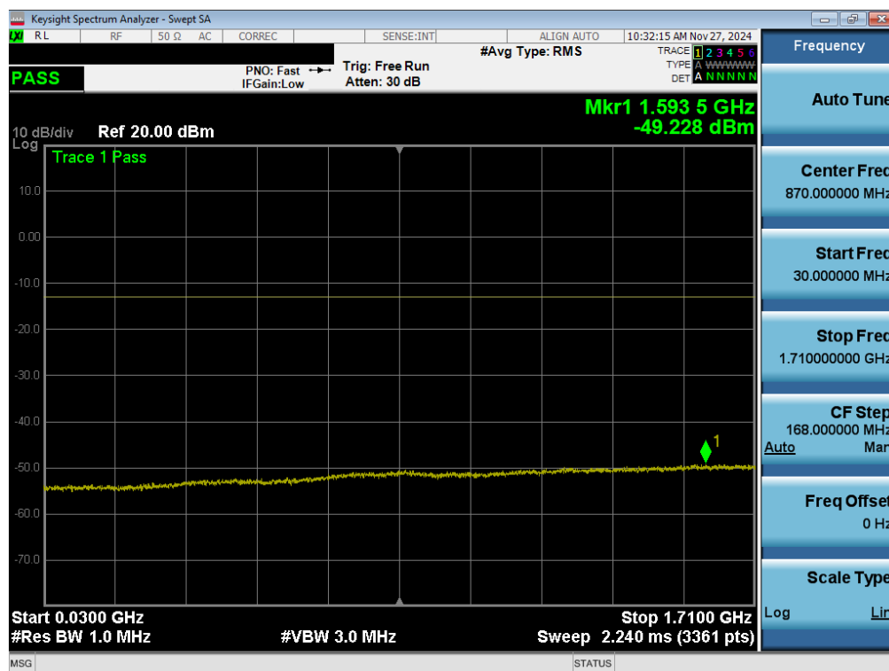
Plot 7-158. Conducted Spurious Plot (LTE Band 66/4 - 20MHz QPSK - 1 RB - Mid Channel – Ant 1)
