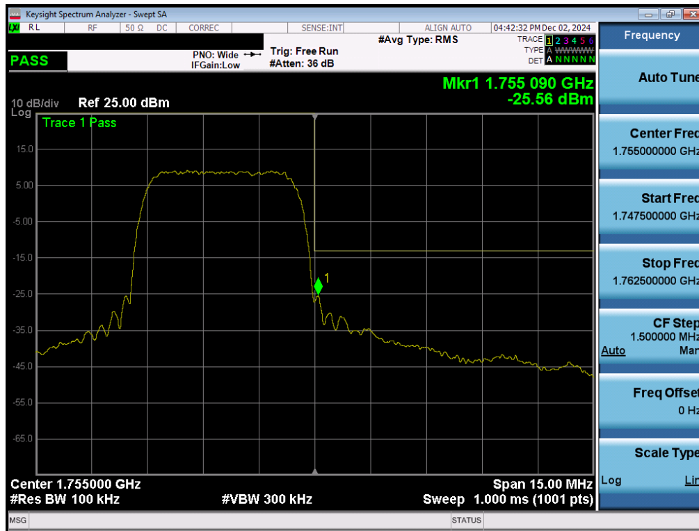
Plot 7-198. Upper Band Edge Plot (WCDMA AWS – Ch. 1513 – Ant 1)
