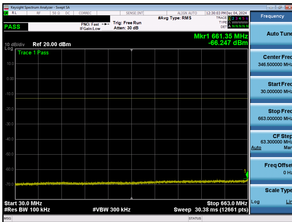
Plot 7-117. Conducted Spurious Plot (LTE Band 71 - 20MHz QPSK - 1 RB - Mid Channel - Ant 5)
