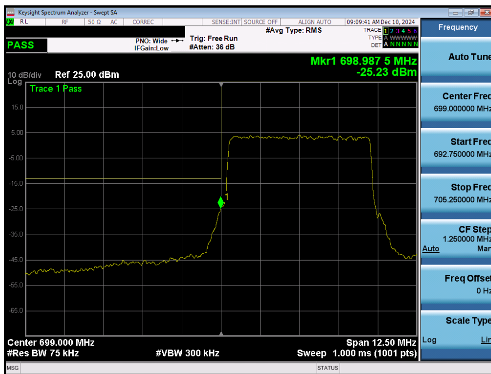
Plot 7-180. Lower Band Edge Plot (NR Band n12 – 5.0MHz - Full RB - Ant 5)
