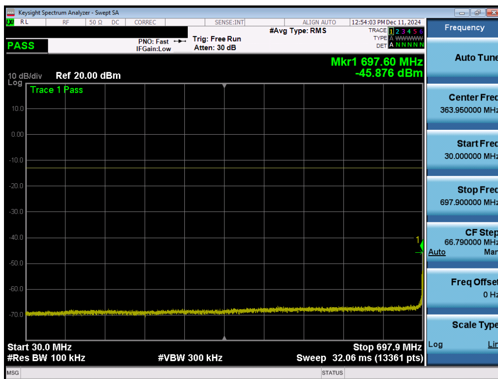
Plot 7-120. Conducted Spurious Plot (LTE Band 12- 10MHz QPSK - 1 RB - Low Channel - Ant 5)
