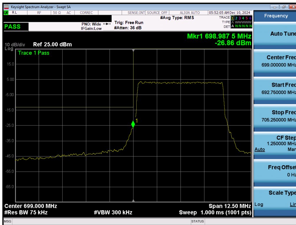
Plot 7-194. Lower Band Edge Plot (NR Band n12 – 5.0MHz - Full RB - Ant 2)
