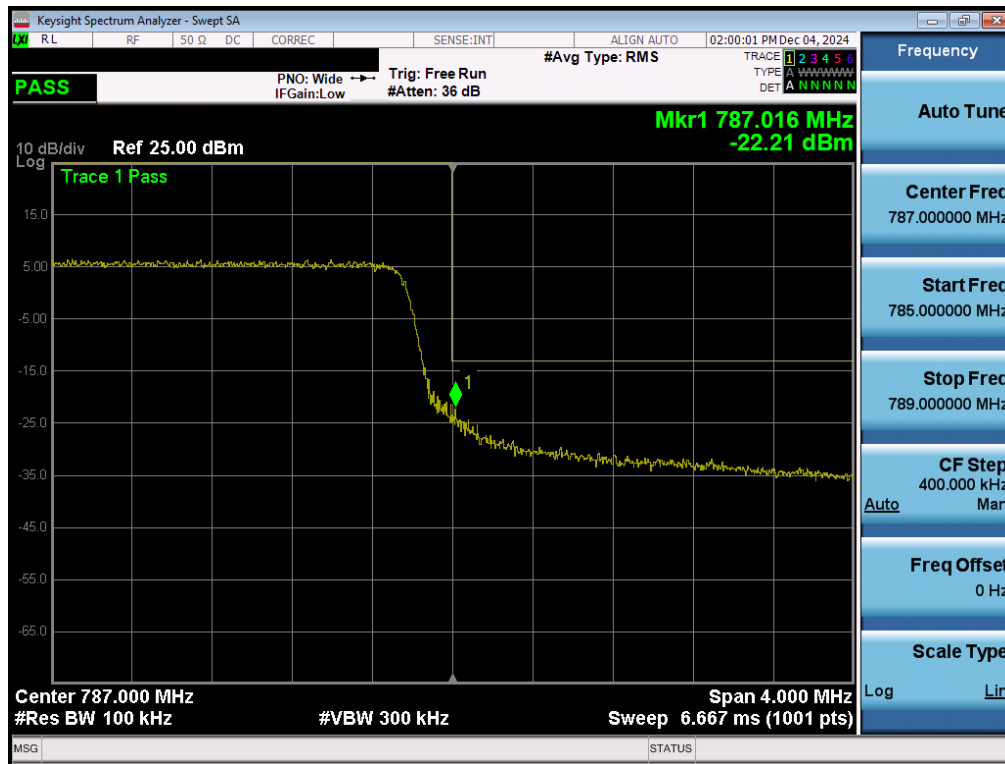
Plot 7-174. Upper Band Edge Plot (LTE Band 13 - 5MHz QPSK - Full RB - Ant 5)
