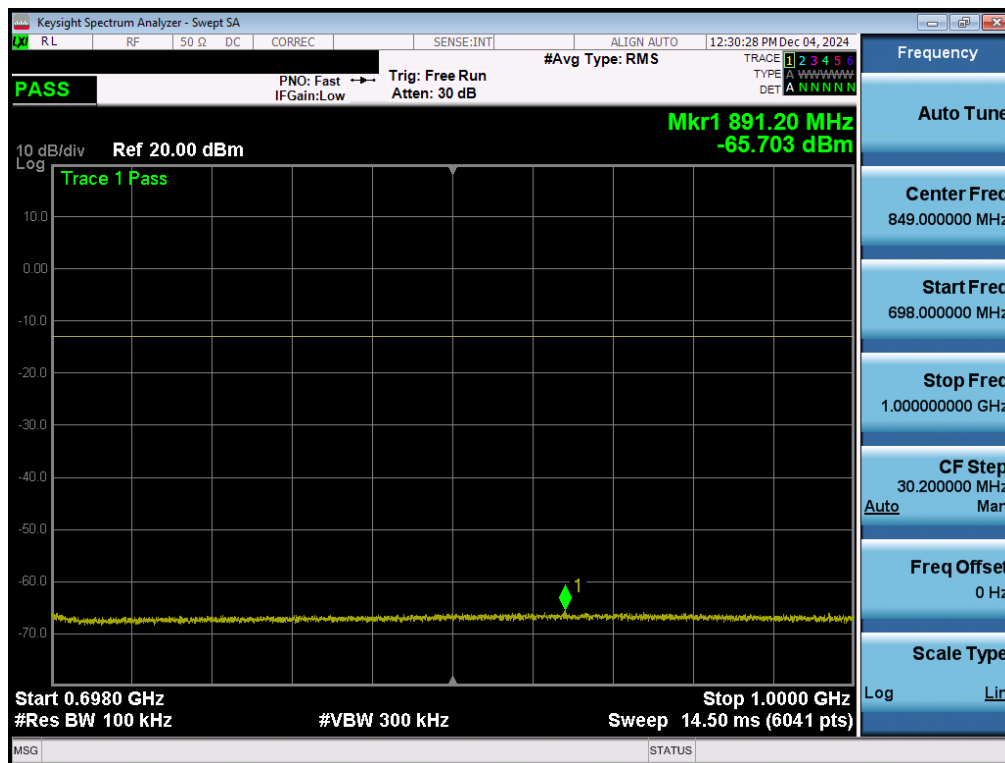
Plot 7-118. Conducted Spurious Plot (LTE Band 71 - 20MHz QPSK - 1 RB - Mid Channel - Ant 5)
