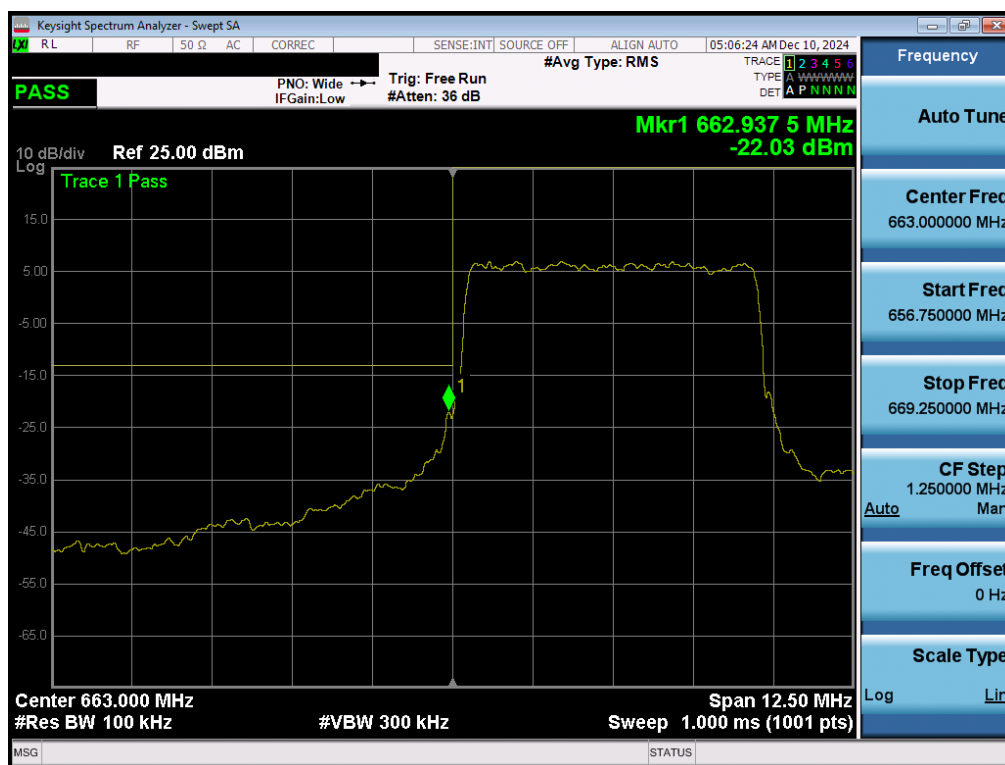
Plot 7-192. Lower Band Edge Plot (NR Band n71 – 5.0MHz - Full RB - Ant 2)
