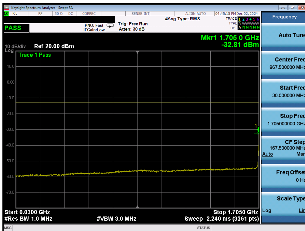
Plot 7-155. Conducted Spurious Plot (WCDMA Ch. 1312- Low Channel - Ant 1)
