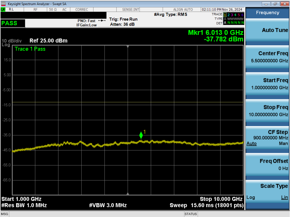
Plot 7-144. Conducted Spurious Plot (LTE Band 13 - 10MHz QPSK - 1 RB - Mid Channel - Ant 2)
