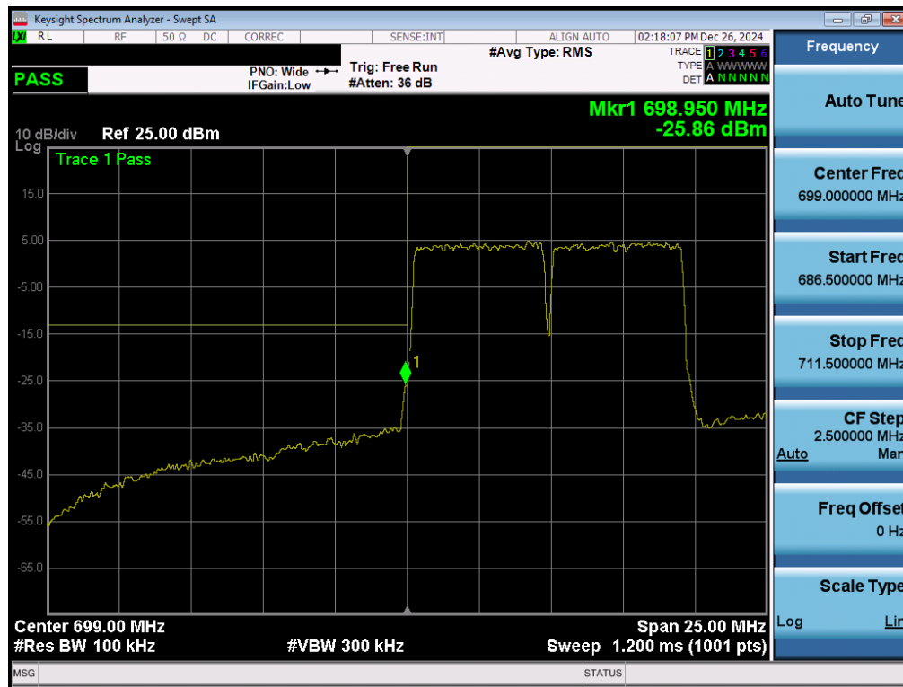
Plot 7-190. Lower Band Edge Plot (ULCA LTE Band 12 - 5+5MHz - Full RB – Ant 2)
