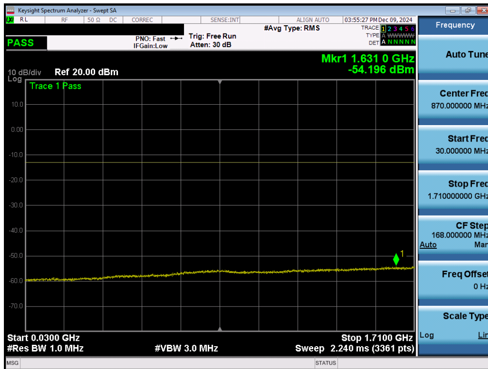
Plot 7-161. Conducted Spurious Plot (NR Band n66 - 40.0MHz - 1 RB - High Channel - Ant 1)
