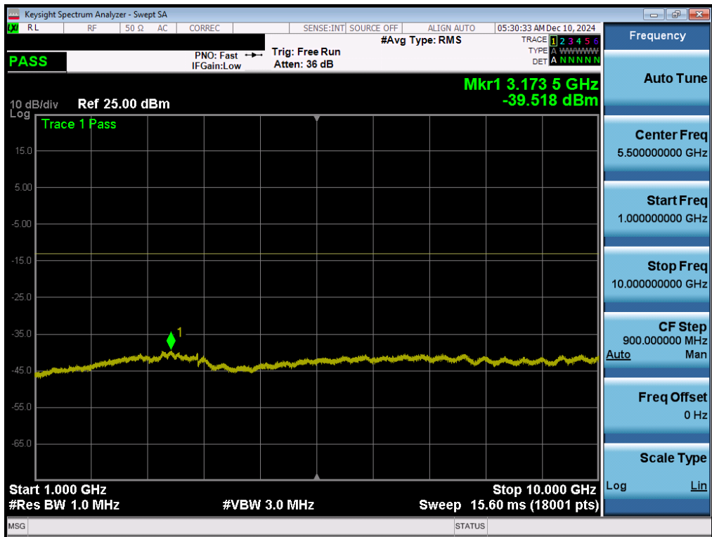
Plot 7-150. Conducted Spurious Plot (NR Band n12 - 15.0MHz - 1 RB - High Channel - Ant 2)
