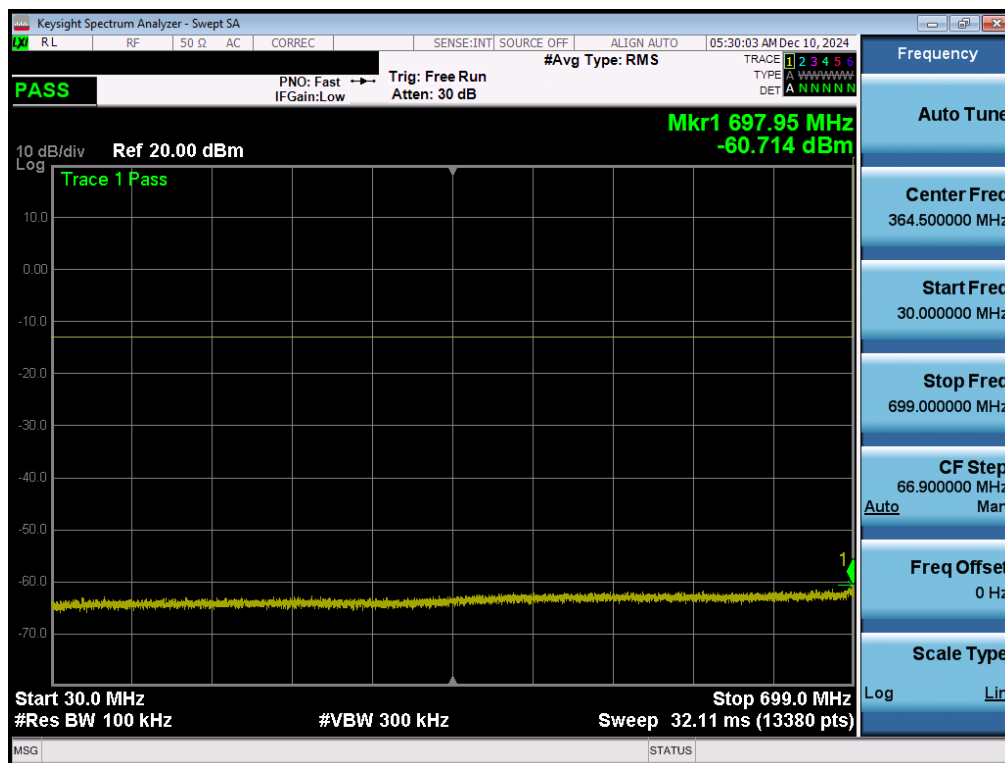
Plot 7-148. Conducted Spurious Plot (NR Band n12 - 15.0MHz - 1 RB - High Channel - Ant 2)
