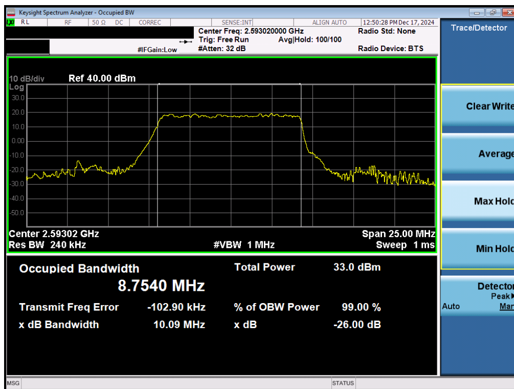
Plot 7-57. Occupied Bandwidth Plot (NR Band n41 - 10MHz \pi/2 BPSK - Full RB - Ant1)
