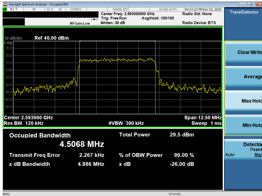
Plot 7-12. Occupied Bandwidth Plot (LTE Band 41(PCI) - 5MHz 16-QAM - Full RB - Ant1)
