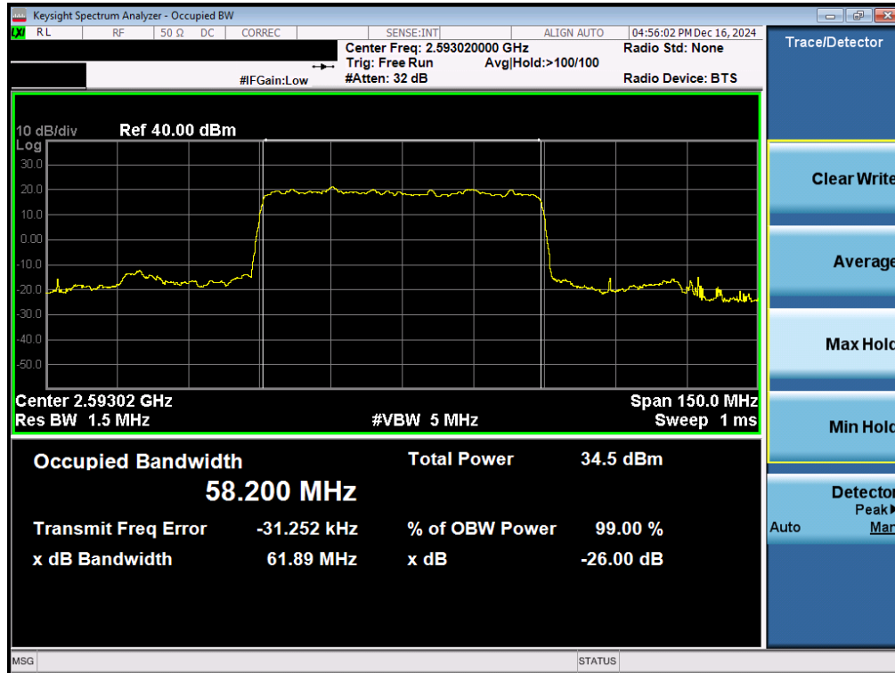
Plot 7-39. Occupied Bandwidth Plot (NR Band n41 - 60MHz \pi/2 BPSK - Full RB - Ant1)
