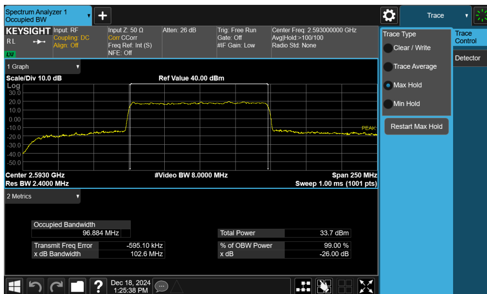
Plot 7-77. Occupied Bandwidth Plot (NR Band n41 - 100MHz QPSK - Full RB - Ant6)
