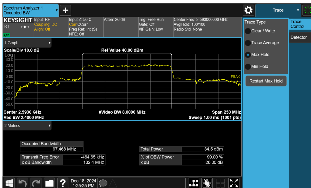
Plot 7-76. Occupied Bandwidth Plot (NR Band n41 - 100MHz \pi/2 BPSK - Full RB - Ant6)
