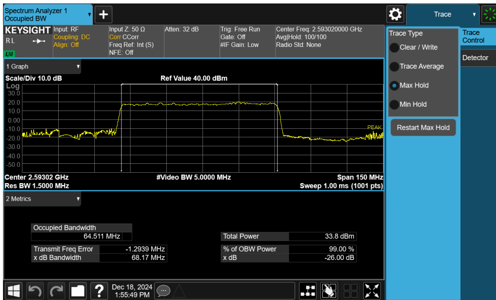
Plot 7-85. Occupied Bandwidth Plot (NR Band n41 - 70MHz \pi/2 BPSK - Full RB - Ant6)
