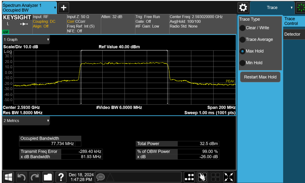
Plot 7-84. Occupied Bandwidth Plot (NR Band n41 - 80MHz 16-QAM - Full RB - Ant6)
