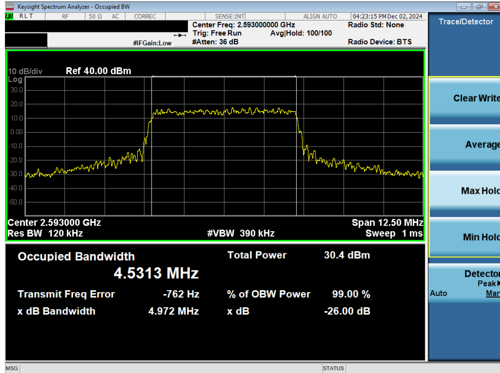
Plot 7-11. Occupied Bandwidth Plot (LTE Band 41(PCI) - 5MHz QPSK - Full RB - Ant1)
