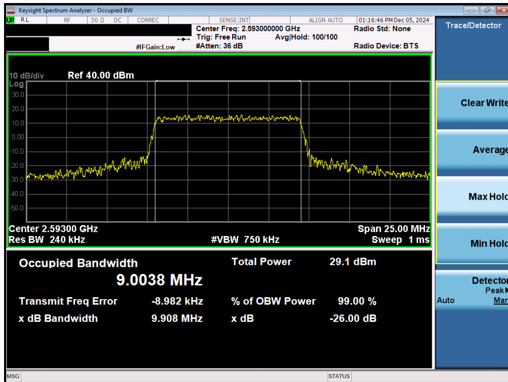
Plot 7-18. Occupied Bandwidth Plot (LTE Band 41(PC3)/38 - 10MHz 16-QAM - Full RB - Ant1)
