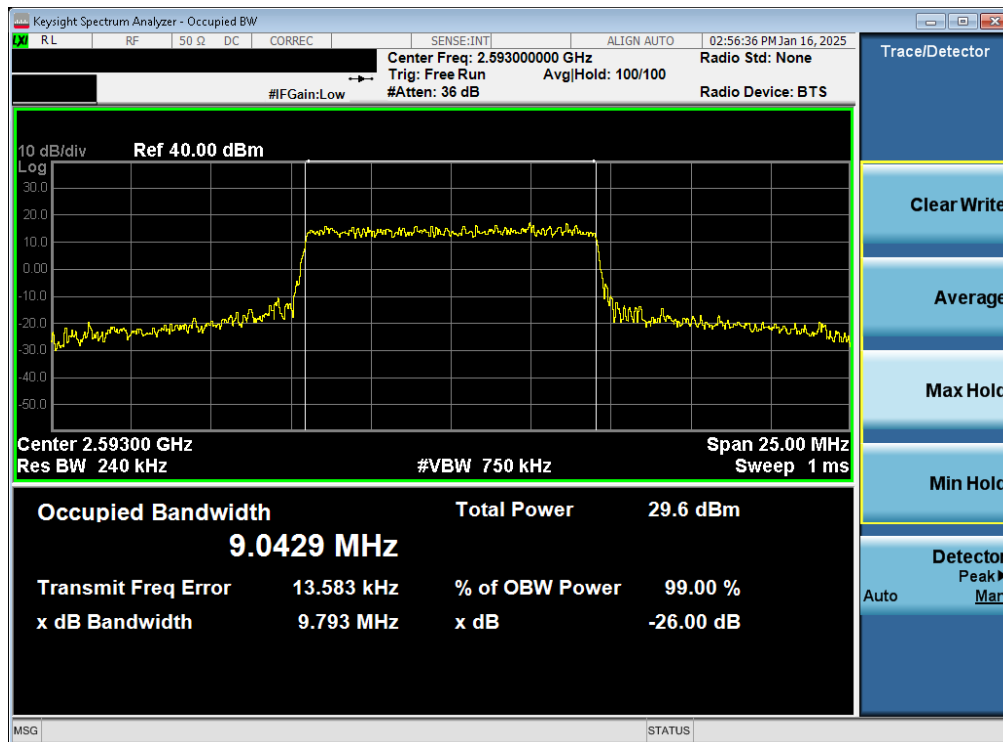
Plot 7-73. Occupied Bandwidth Plot (LTE Band 41(PC3)/38 - 10MHz 16-QAM - Full RB - Ant6)
