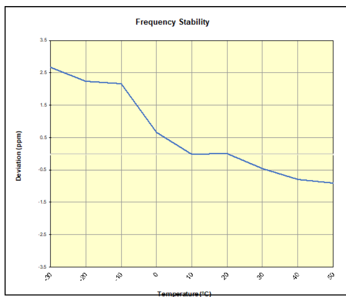
Plot 7-225. LTE Band 30 Frequency Stability Chart
