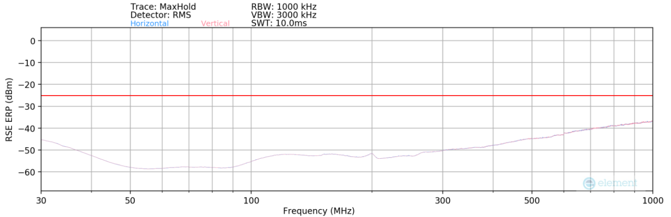
Plot 7-199. Radiated Spurious Plot Below 1GHz (NR Band n41PC2) – Ant1)
