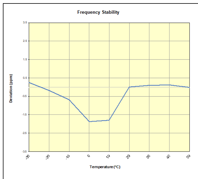
Plot 7-226. LTE Band 41(PC2) Frequency Stability Chart
