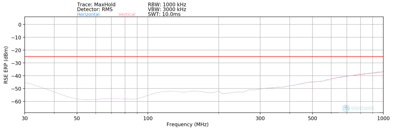
Plot 7-205. Radiated Spurious Plot Below 1GHz (ULCA LTE B41(PC3) – Ant1)
