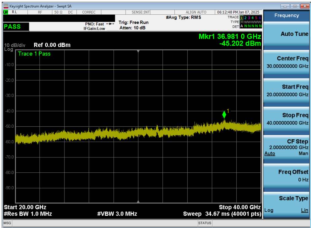
Plot 7-298. Conducted Spurious Plot (NR Band n77 DoD - 100MHz QPSK - RB Size 1, RB Offset 136 - Mid Channel – SRS Ant4)
