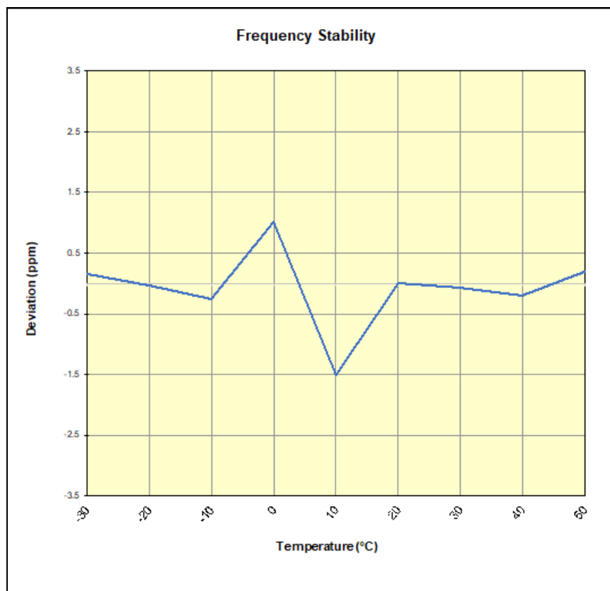
Plot 7-131. LTE Band 48 Frequency Stability Chart
