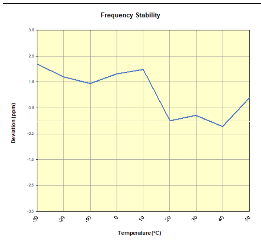
Plot 7-132. NR Band n48 Frequency Stability Chart
