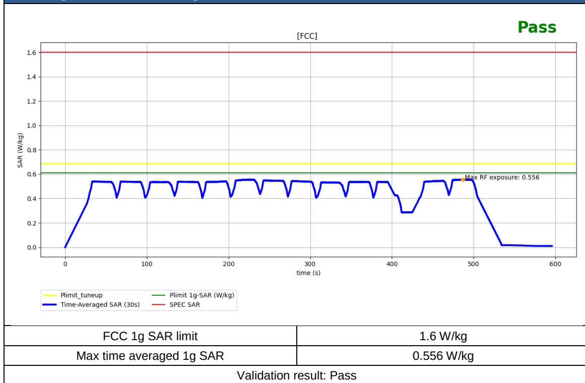
Figure 6-18-2 Time-averaged 6G SAR measurement for Wi-Fi TA-SAR test scenario 1-1
