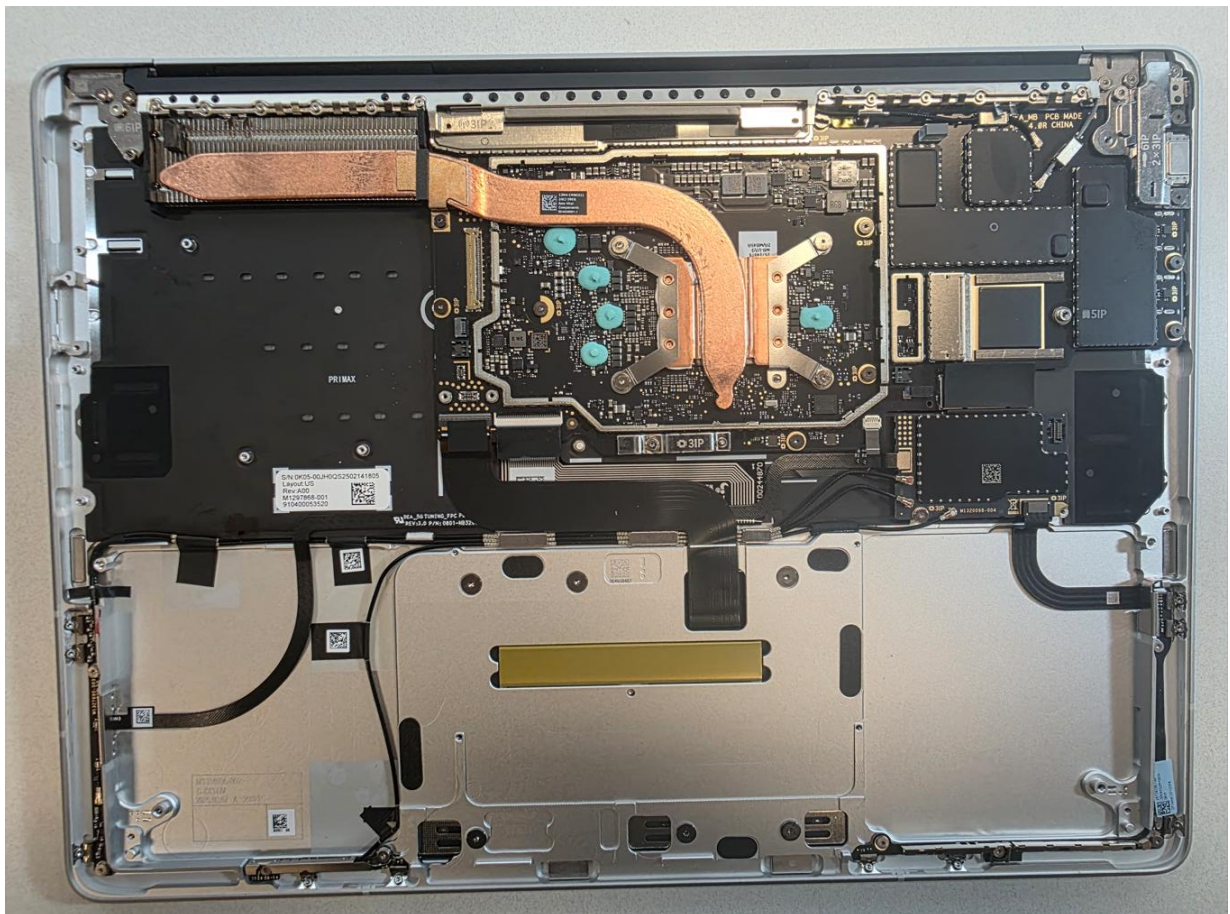
Model 2119 Internal Photographs
