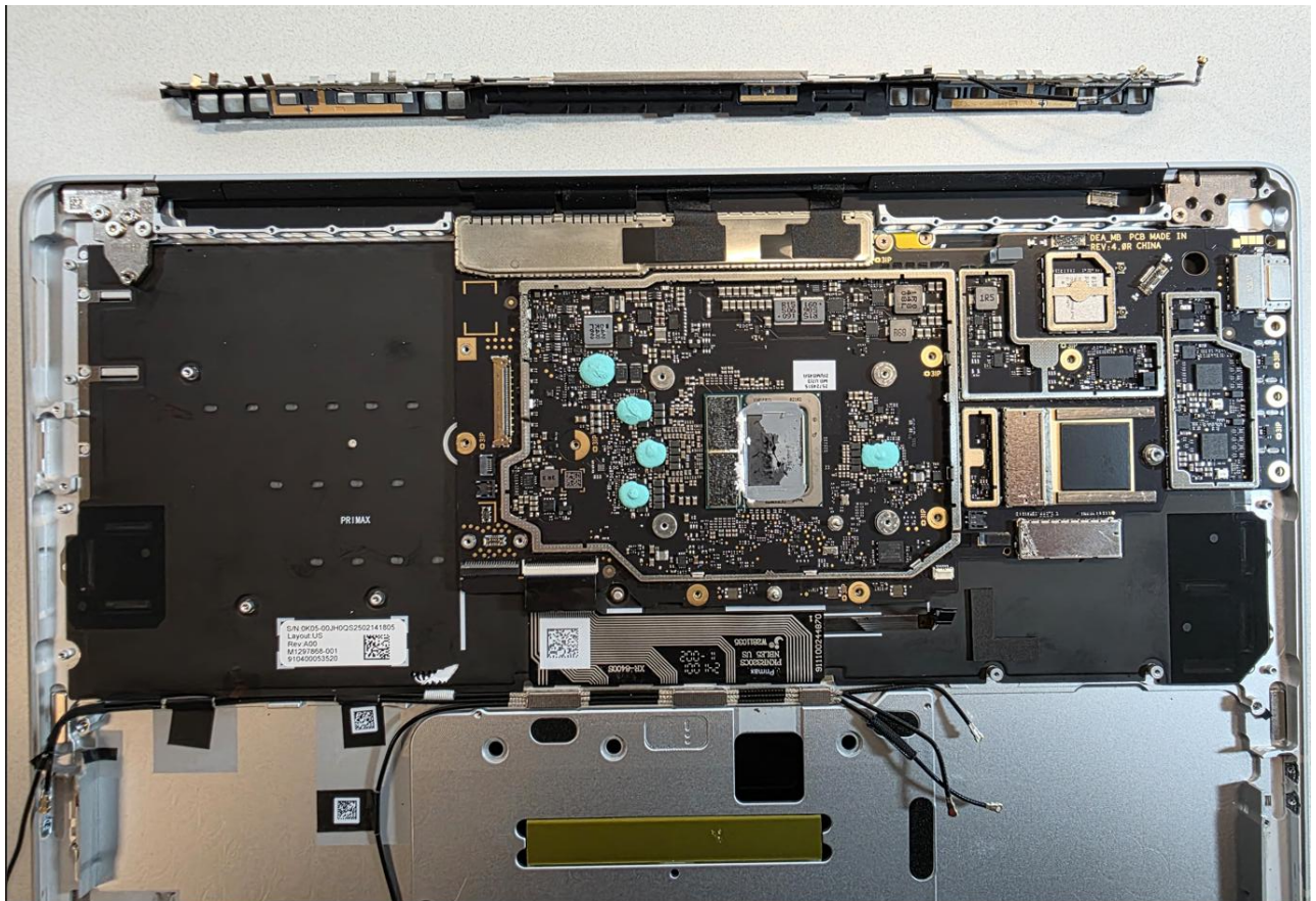
Model 2119 Internal Photographs
