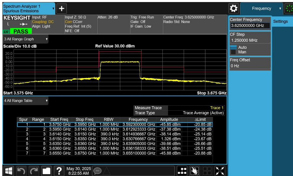
Plot 7-105. Channel - Ant6 Edge Plot (LTE Band 48 - 20MHz QPSK - Mid Channel - Ant6)
