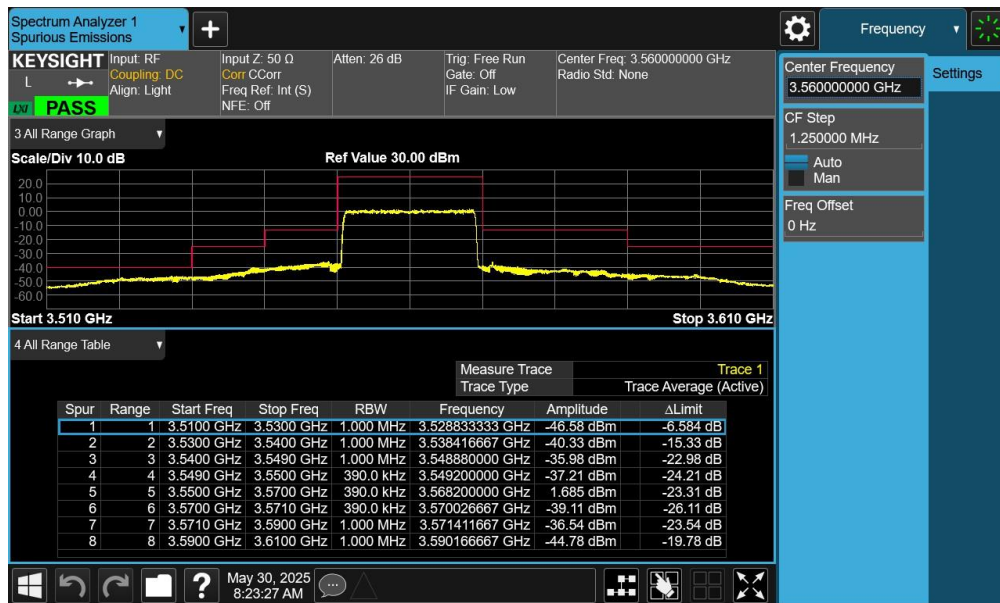
Plot 7-104. Channel - Ant6 Edge Plot (LTE Band 48 - 20MHz QPSK - Low Channel - Ant6)
