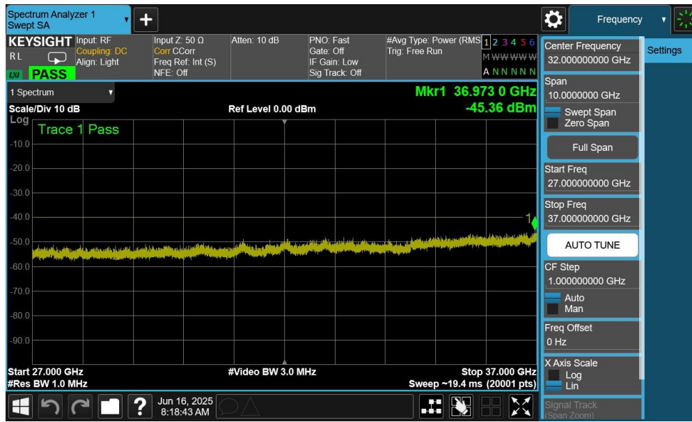
Plot 7-75. Conducted Spurious Plot (ULCA LB48 - 20+20MHz QPSK - High Channel - Ant6)
