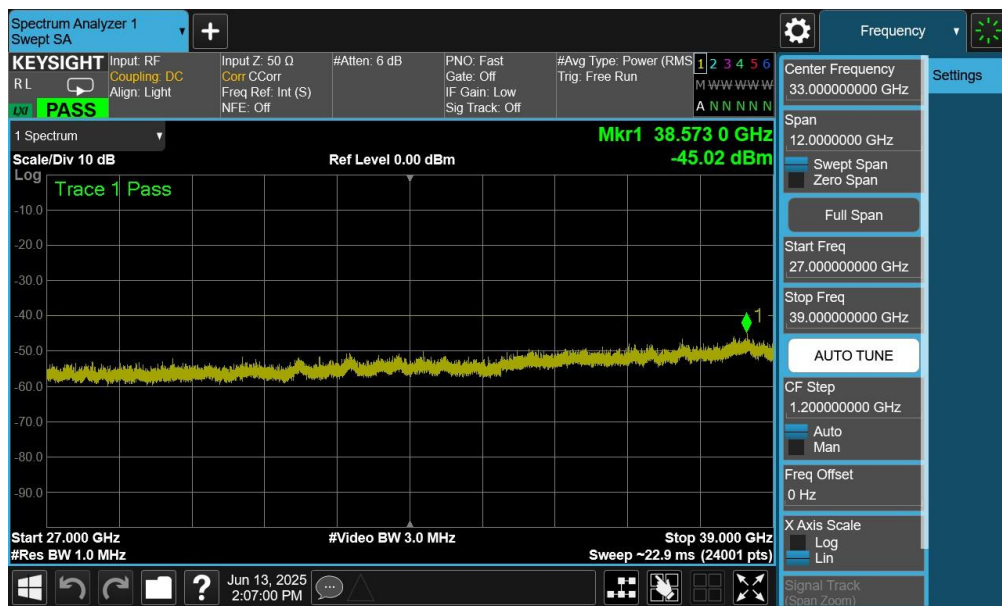
Plot 7-79. Conducted Spurious Plot (NR Band n48 - 40MHz QPSK - High Channel - Ant6)
