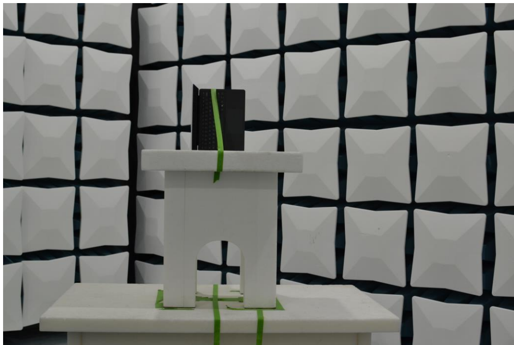
Figure 14. Test Setup – Y Position – 1GHz-40GHz – Half Open
