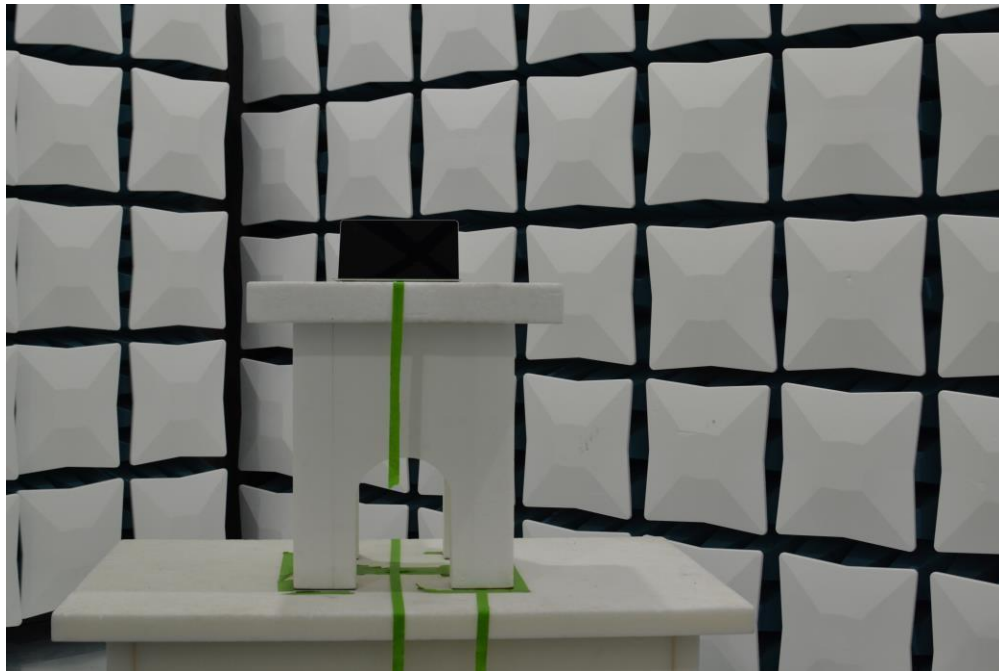
Figure 7. Test Setup – X Position – 1GHz-40GHz – Open
