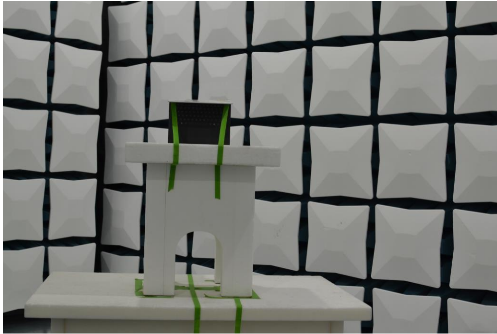
Figure 15. Test Setup – Z Position – 1GHz-40GHz – Half Open
