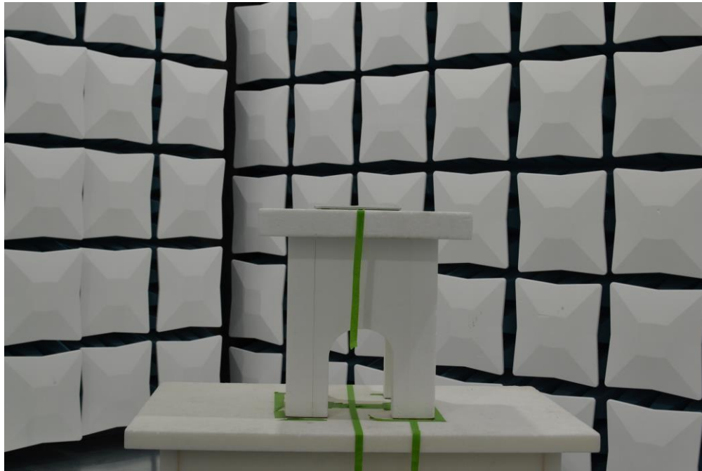
Figure 1. Test Setup – X Position – 1GHz-40GHz – Closed
