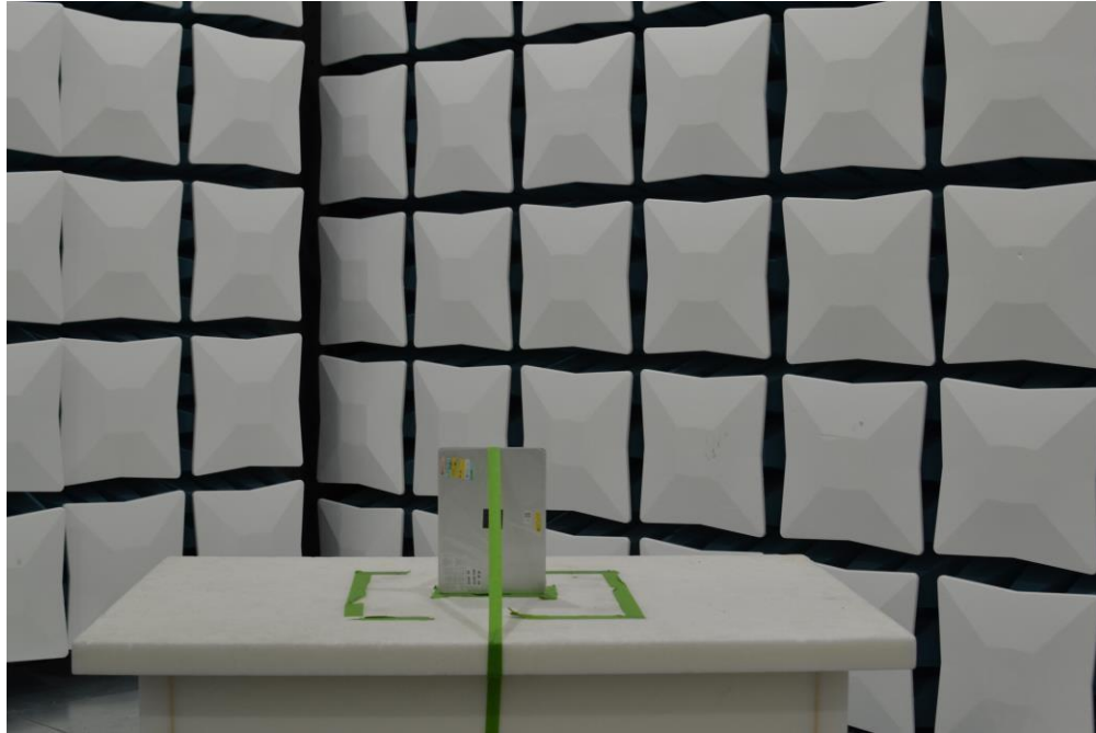
Figure 5. Test Setup – Y Position – 30MHz-1GHz – Closed
