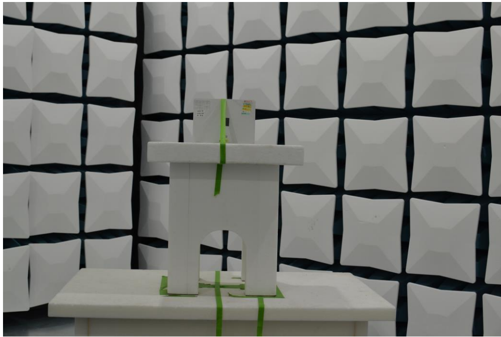
Figure 3. Test Setup – Z Position – 1GHz-40GHz – Closed
