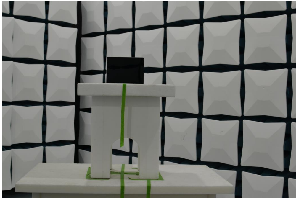
Figure 13. Test Setup – X Position – 1GHz-40GHz – Half Open
