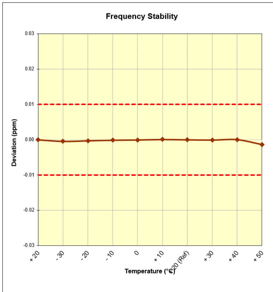
Figure 7-4. Frequency Stability Plot
