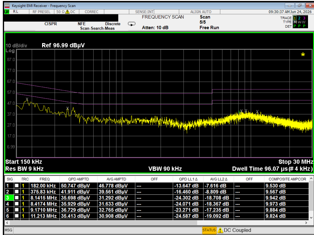
Plot 7-8. Line-Conducted Test Plot (L1) - RFID
