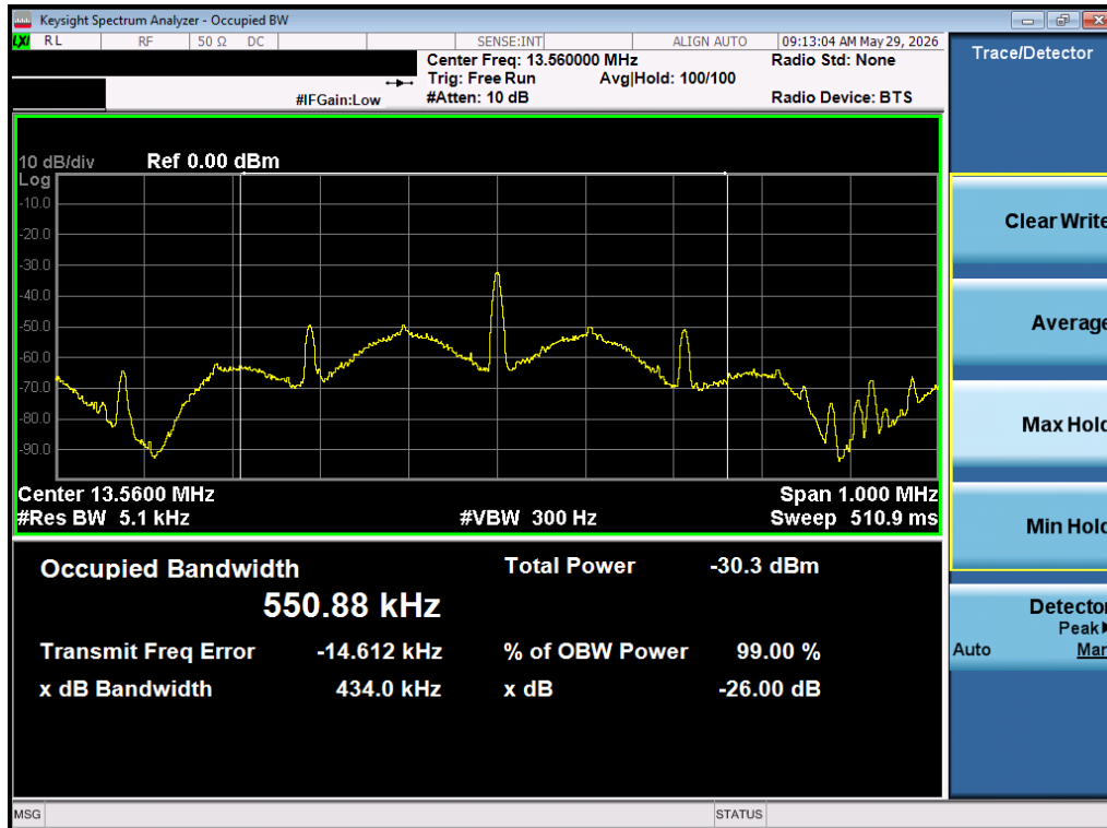
Figure 7-2. Occupied Bandwidth Plot – RFID
