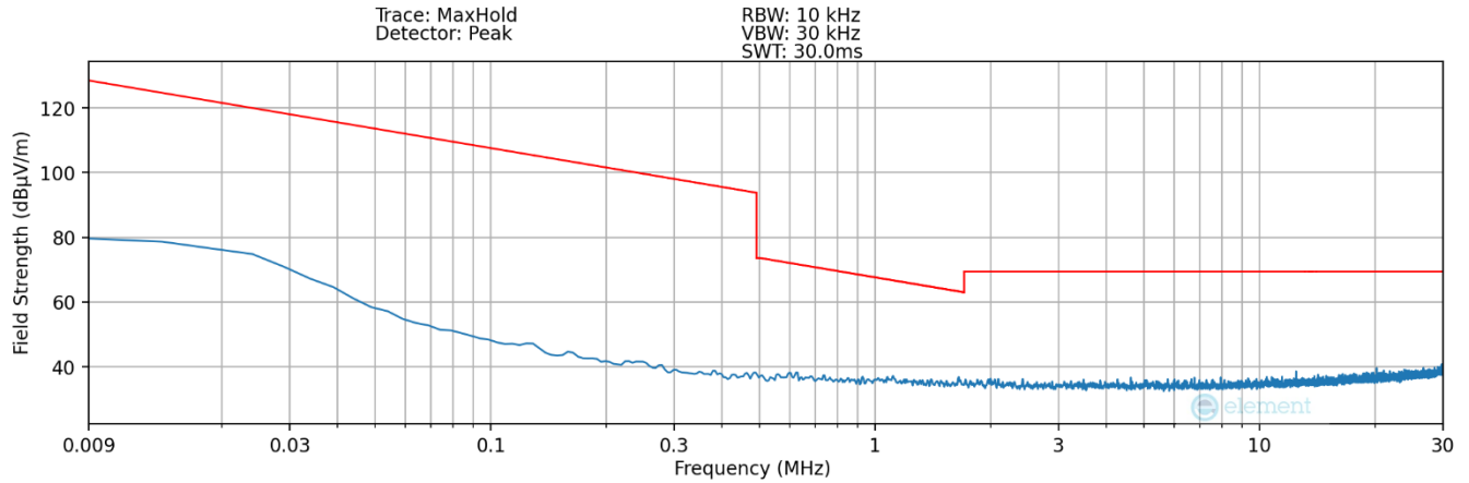
Plot 7-5. Radiated Spurious Plot 9kHz – 30MHz (Pol. X – Device to Pen)
