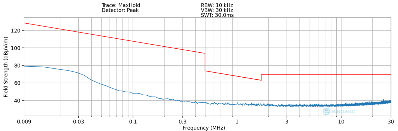
Plot 7-7. Radiated Spurious Plot 9kHz – 30MHz (Pol. Z– Device to Pen)
