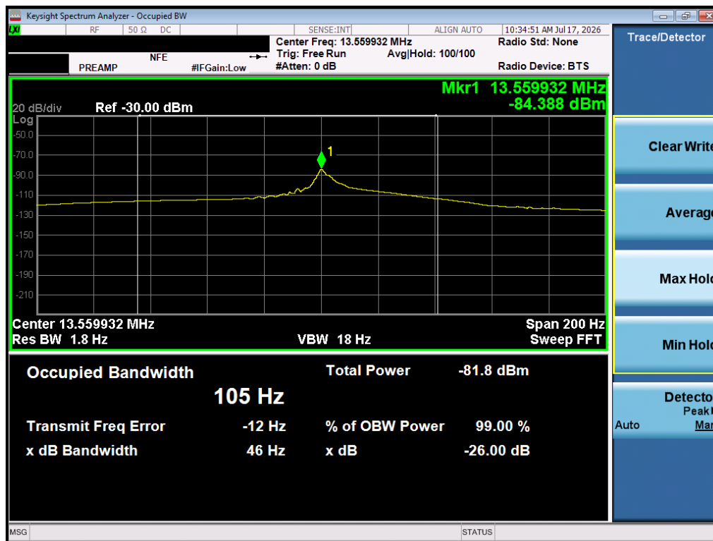
Figure 7-3. Occupied Bandwidth Plot – Device to Pen
