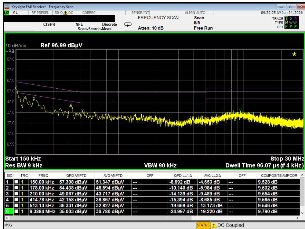
Plot 7-9. Line-Conducted Test Plot (N) – RFID
