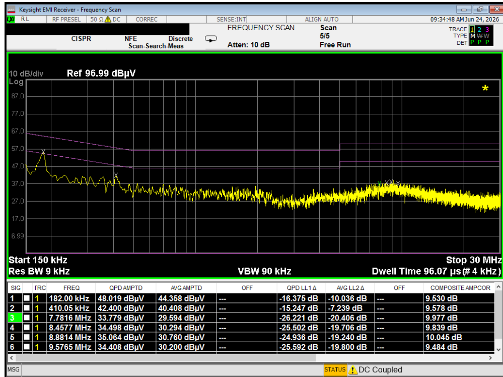
Plot 7-11. Line-Conducted Test Plot (N) - WPT
