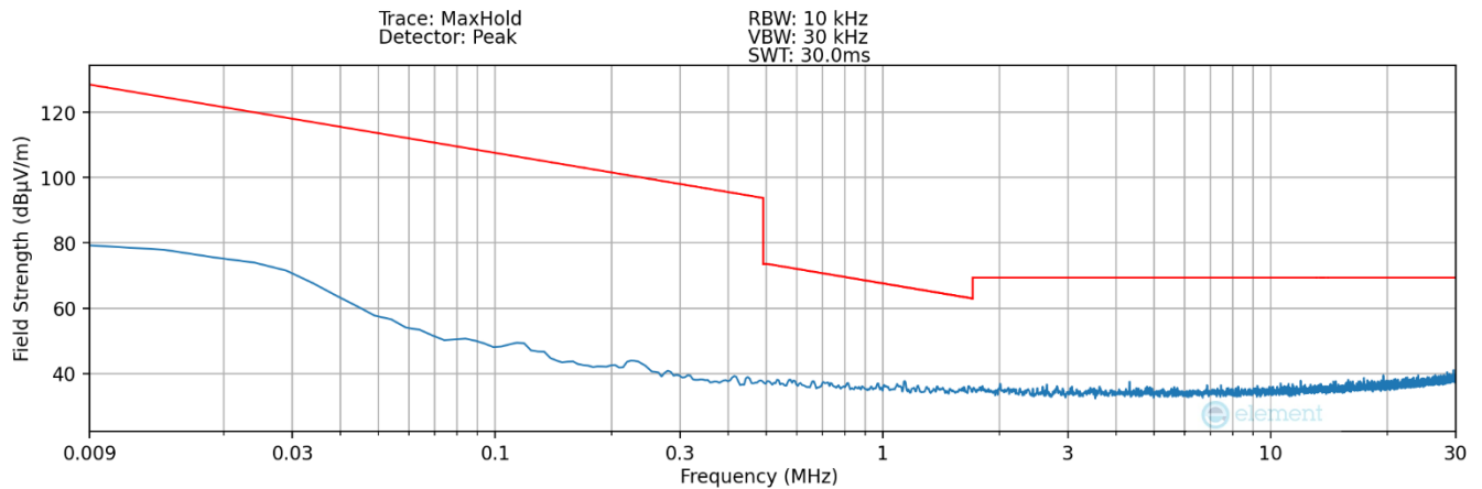
Plot 7-6Radiated Spurious Plot 9kHz – 30MHz (Pol. Y – Device to Pen)
