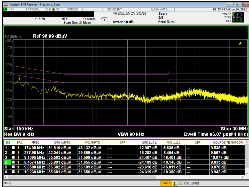
Plot 7-10. Line-Conducted Test Plot (L1) - WPT
