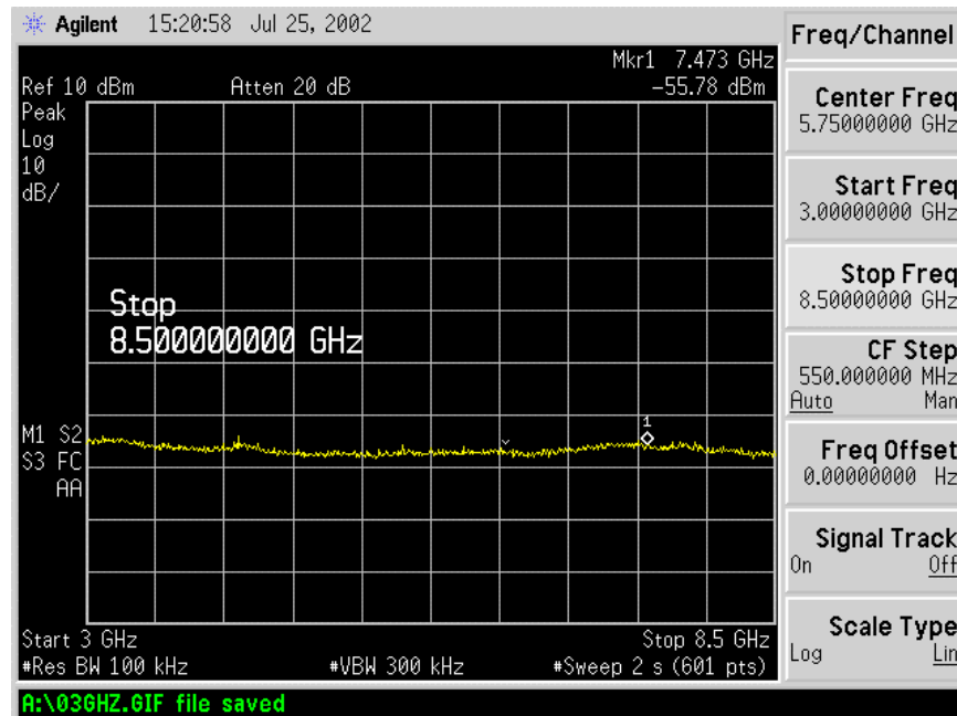
Figure 6.7-6: 3.0 – 8.5GHz Spectrum
