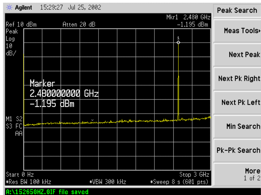
Figure 6.7-9: 0 - 3.0GHz Spectrum
