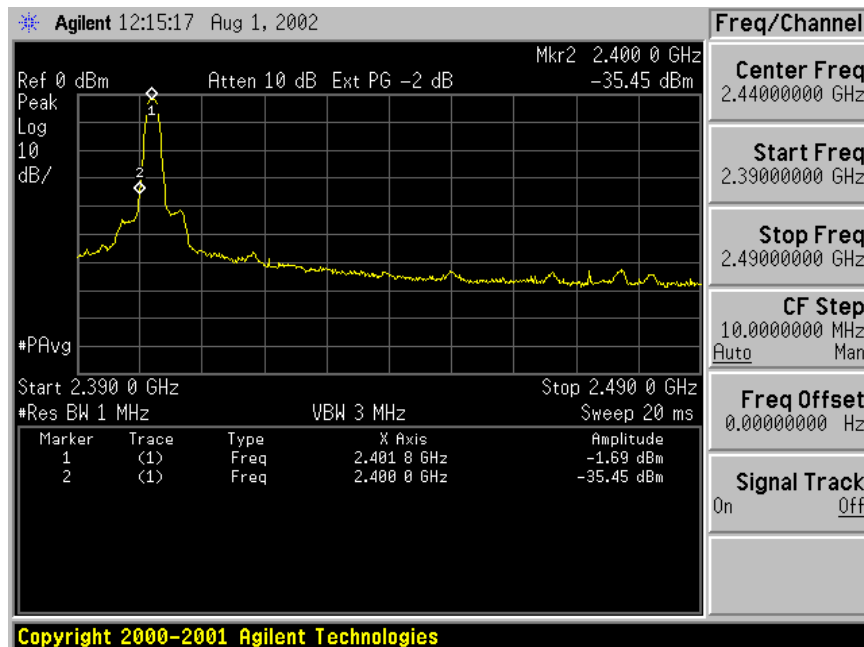
Figure 6.6-1: Lower Band-edge measurement
