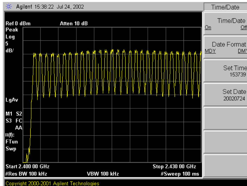
Figure 6.2-1 Channels in the Frequency range 2.400-2.430GHz
