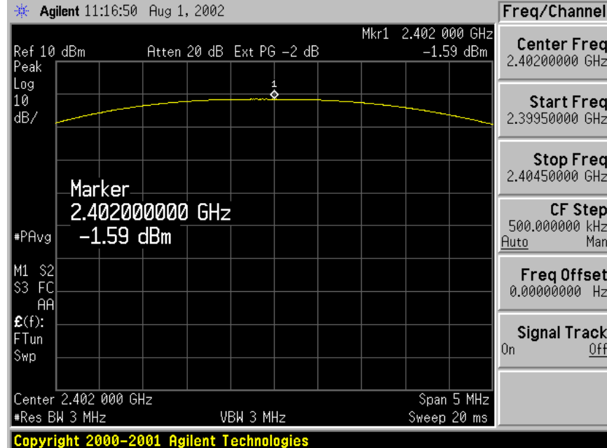
Figure 6.5-1: Power Output on 2402 MHz
