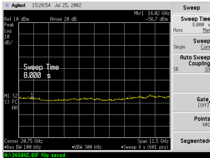
Figure 6.7-8: 15.0 – 26.5GHz Spectrum
