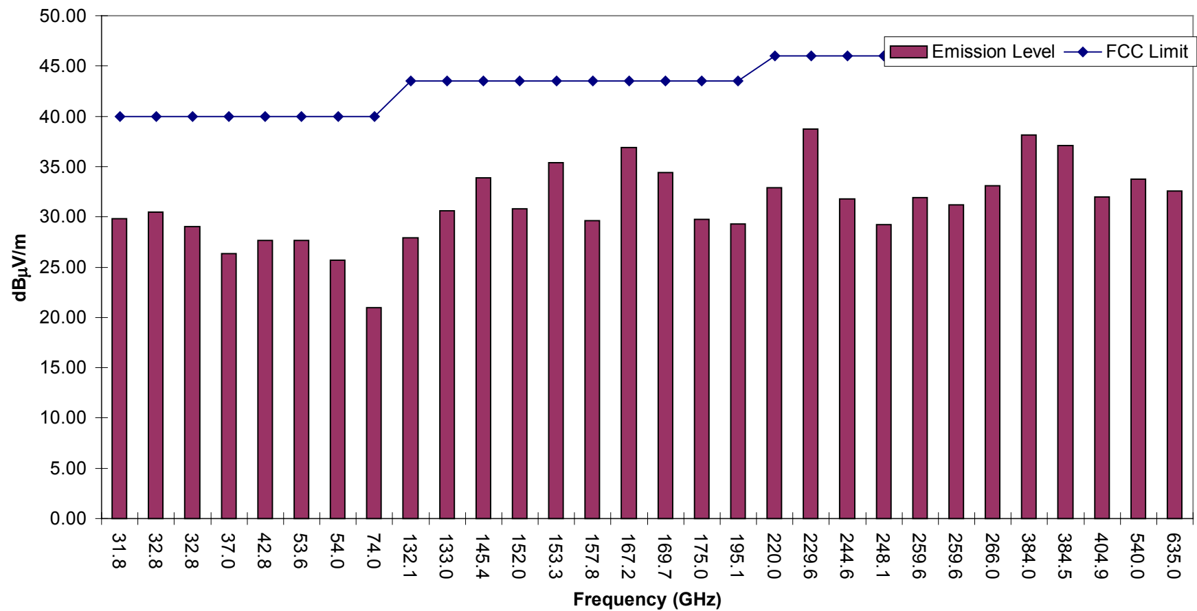
Plot of Spurious Emissions from EUT
