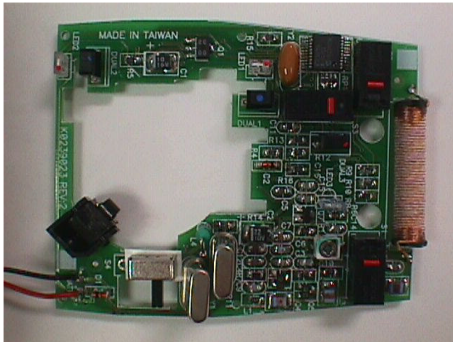
FIGURE 5: Mouse PCB component side
