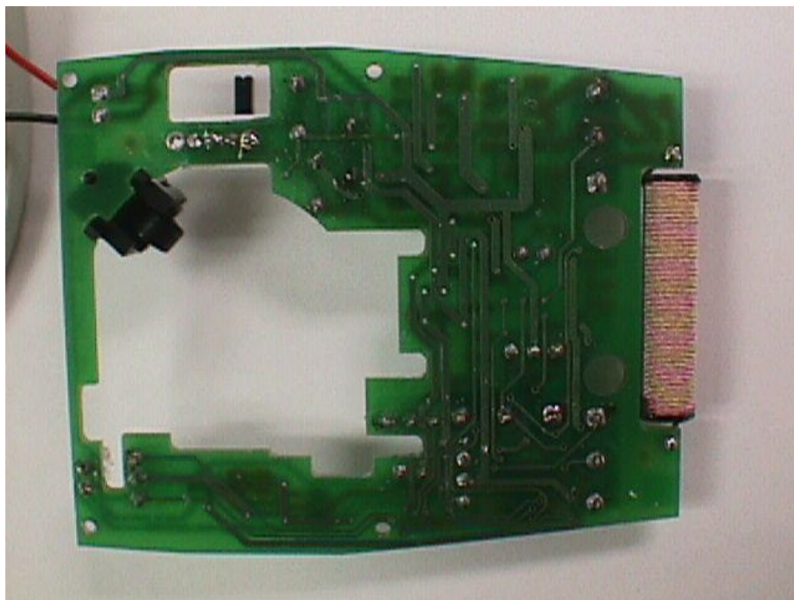
FIGURE 6: Mouse PCB solder side
