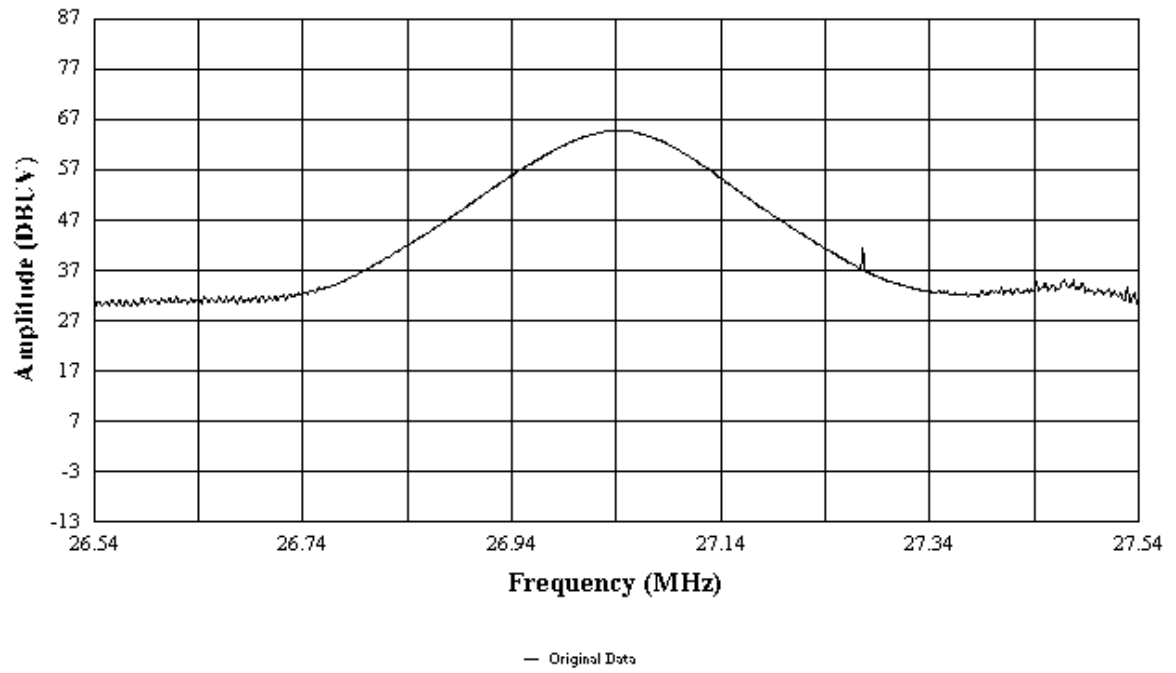
FIGURE 30: MACH99#4 CHANNEL 1 AT 27.042M PS2 Plot
