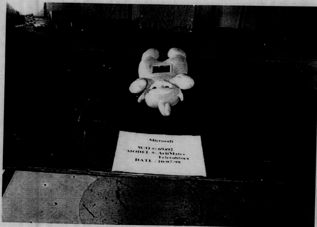
Radiated Emissions – Horizontal Back View
