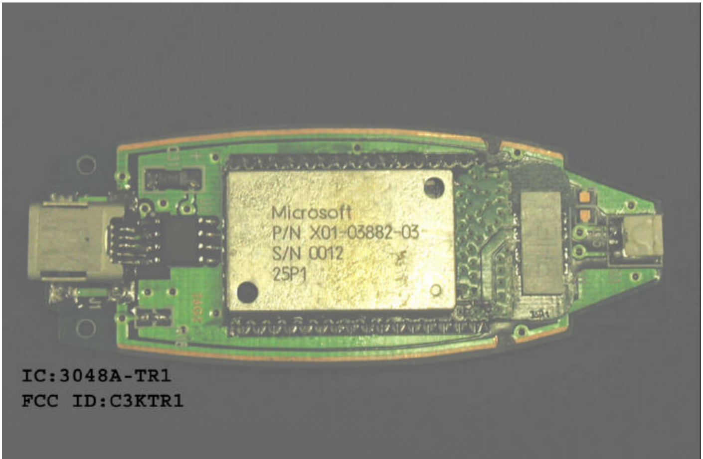
Exhibit 7 Internal Photos C3KTR1 Lapis Dongle
