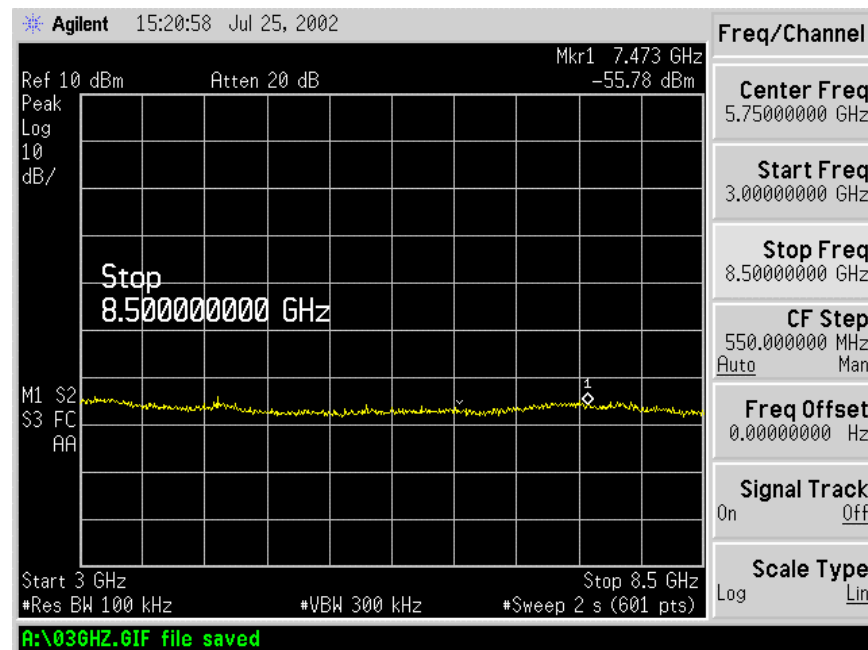
Figure 6.7-6: 3.0 – 8.5GHz Spectrum
