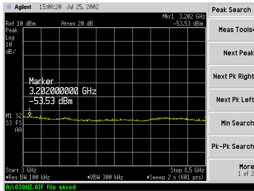
Figure 6.7-2: 3.0 – 8.5GHz Spectrum
