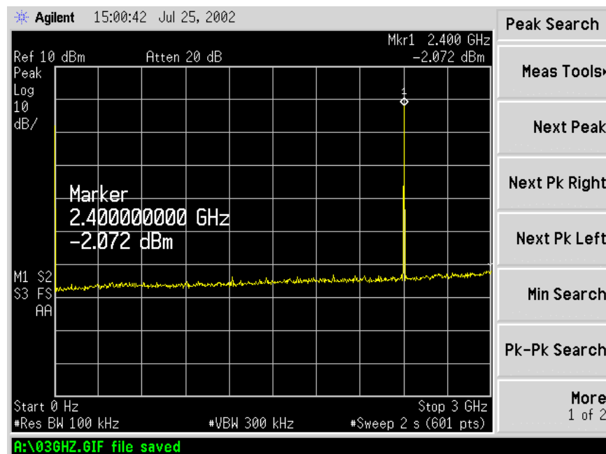
Figure 6.7-1: 0 - 3.0GHz Spectrum
