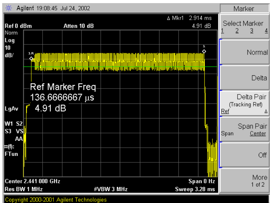
Figure 6.3-3: DH5 Mode Dwell Time
