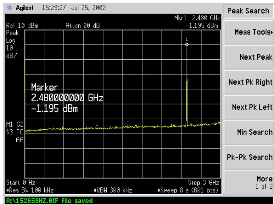
Figure 6.7-9: 0 - 3.0GHz Spectrum
