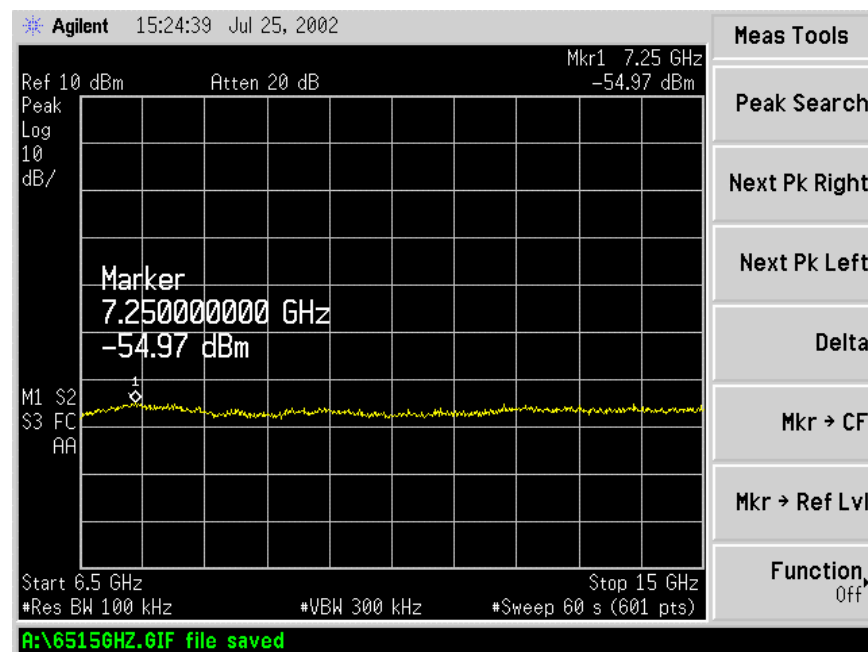
Figure 6.7-7: 6.5 – 15.0GHz Spectrum
