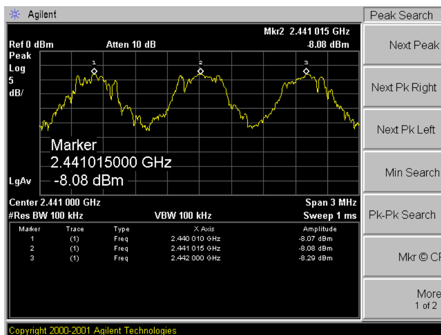
Figure 6.1-1: Carrier Frequency Separation
