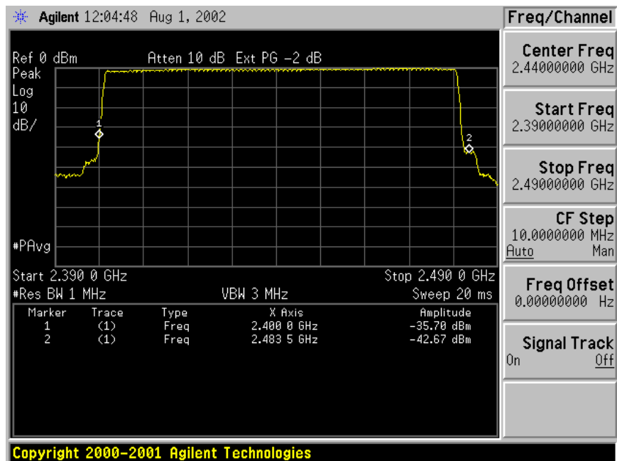
Figure 6.6-3: Plot of Hopping function enabled
