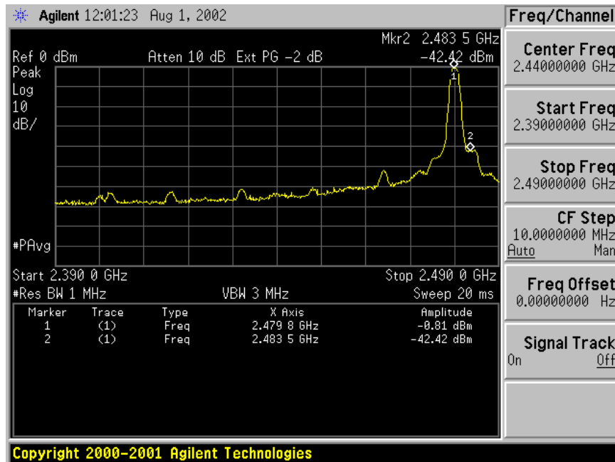
Figure 6.6-2: Upper Band-edge measurement
