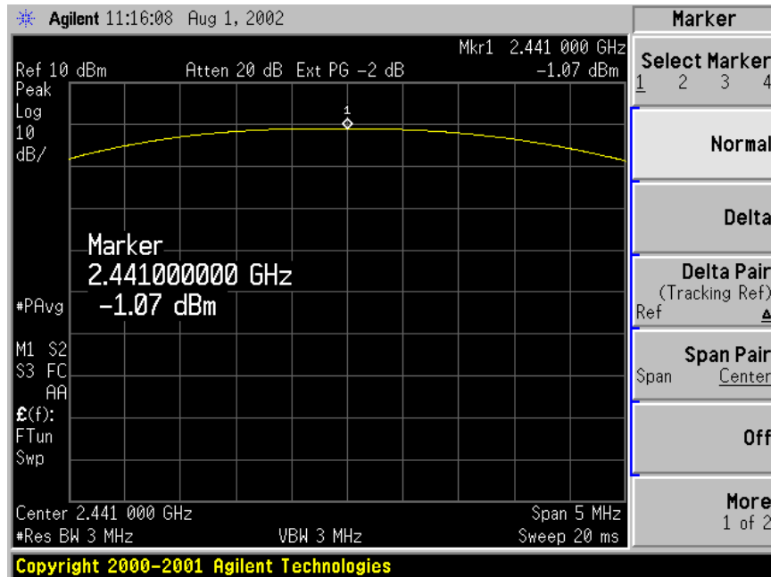
Figure 6.5-1: Power Output on 2441 MHz
