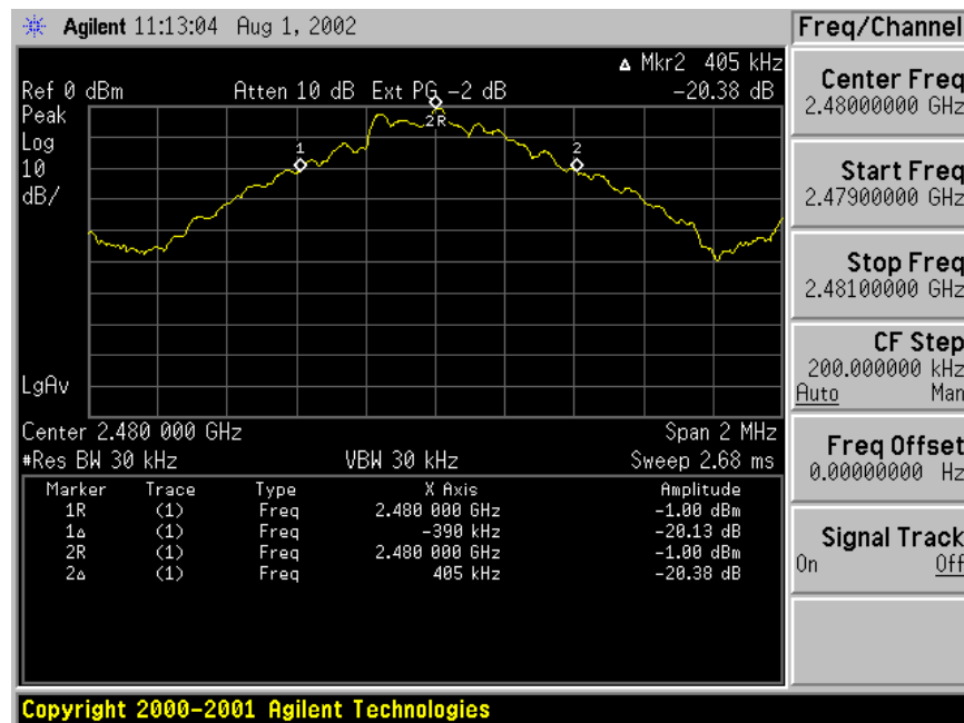
Figure 6.4-1: Bandwidth of the 2480 MHz channel
