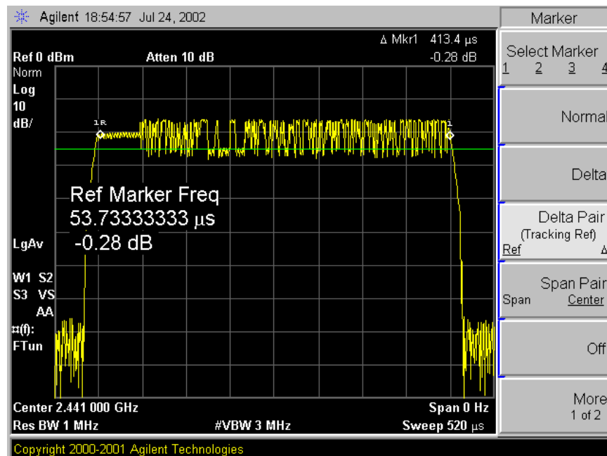
Figure 6.3-1: DH1 Mode Dwell Time
