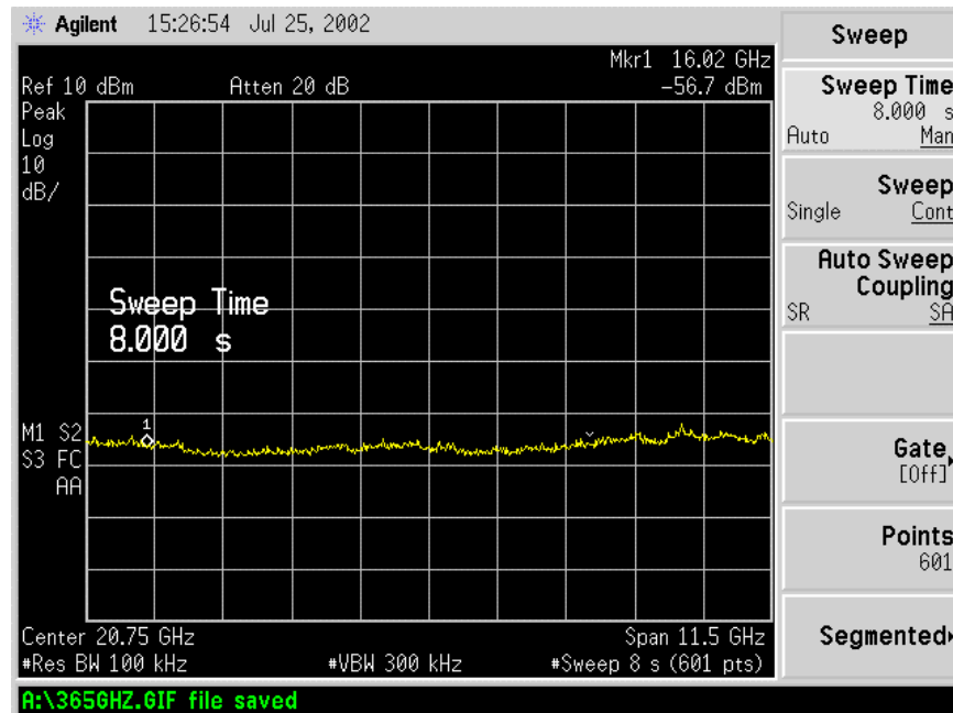
Figure 6.7-8: 15.0 – 26.5GHz Spectrum
