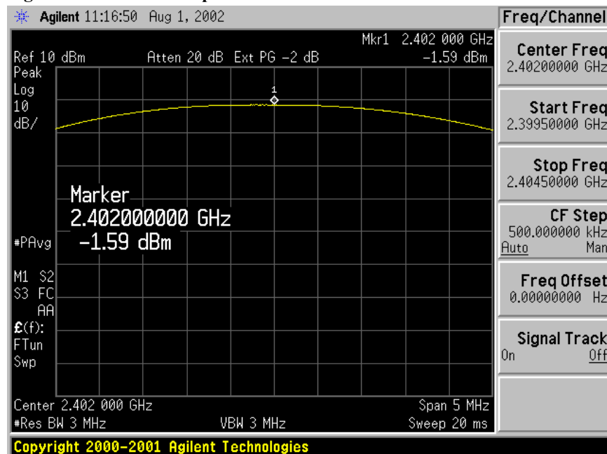
Figure 6.5-1: Power Output on 2402 MHz
