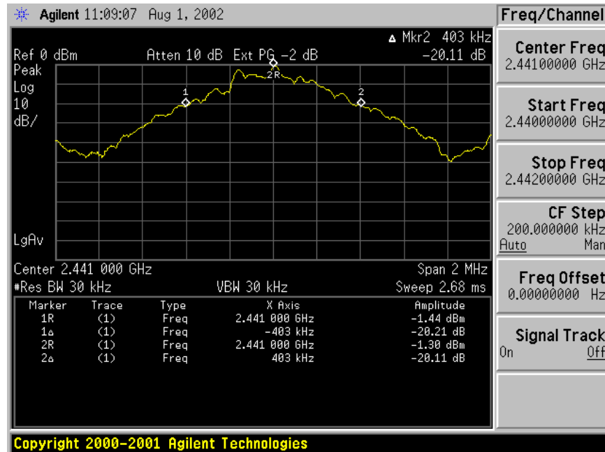
Figure 6.4-2: Bandwidth of the 2441 MHz channel
