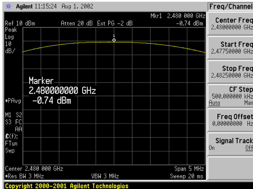
Figure 6.5-1: Power Output on 2480 MHz
