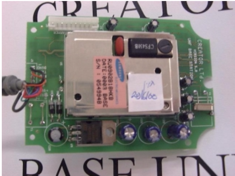
Analog Base PCB Component Side
