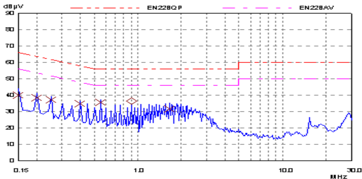
Figure 2 - Line 2 scan
