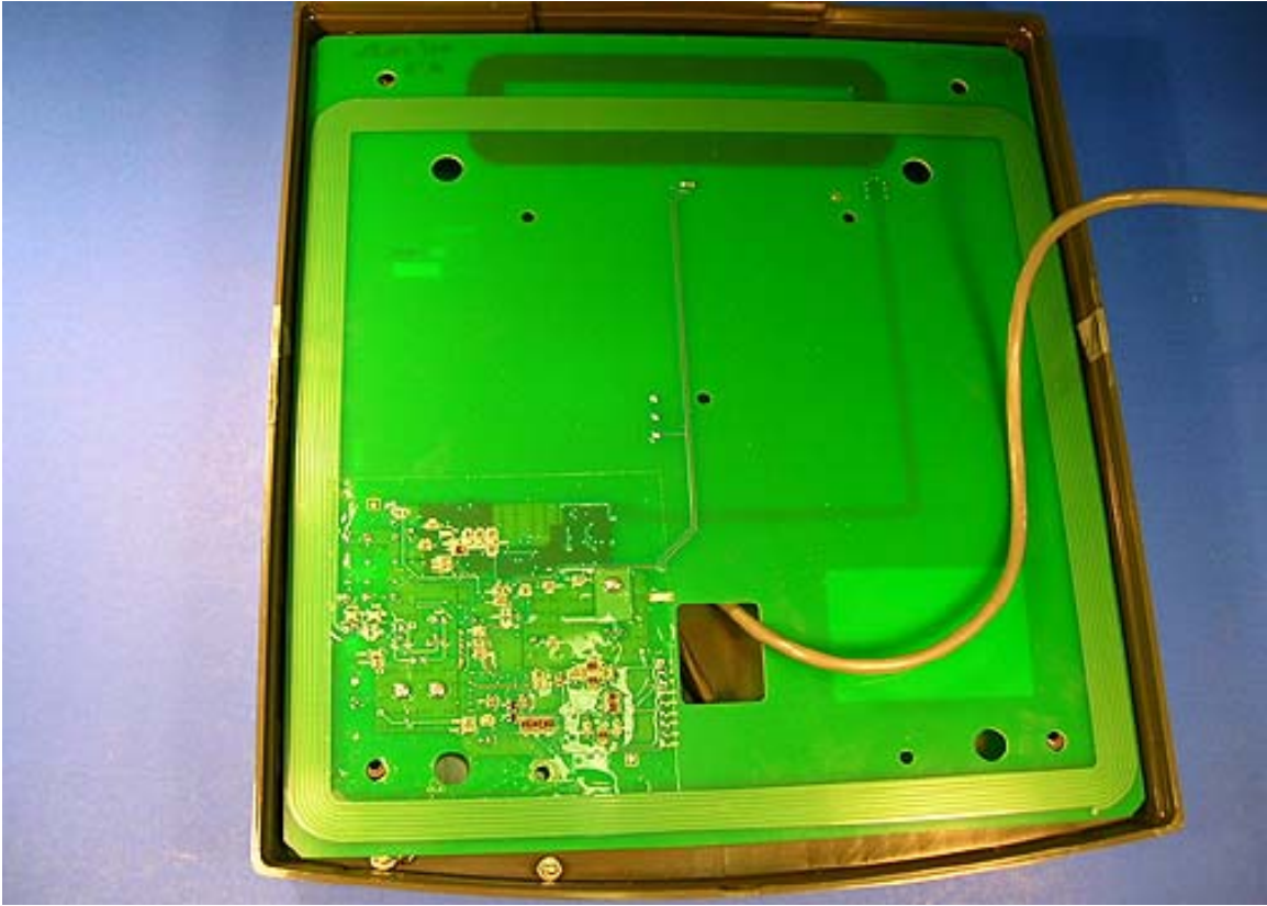
PCB Back
