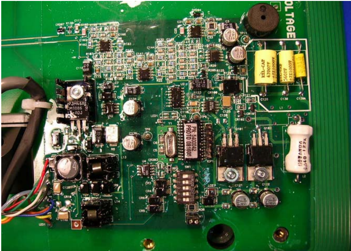
PCB Components Upper Right
