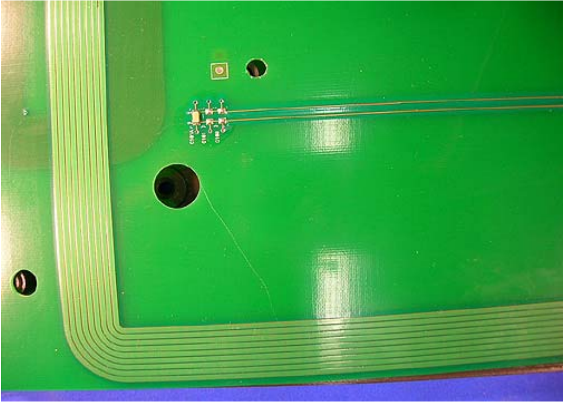
PCB Components Lower Left
