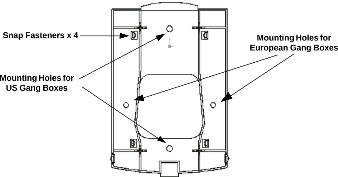
Figure 9: DR4201 Mounting Holes Indicated
