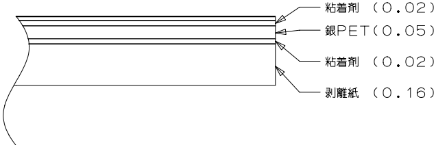
側面詳細 (SCALE 50/1)
