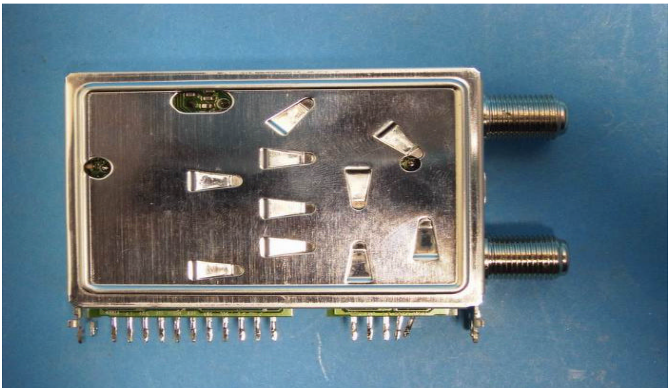
Rear View
