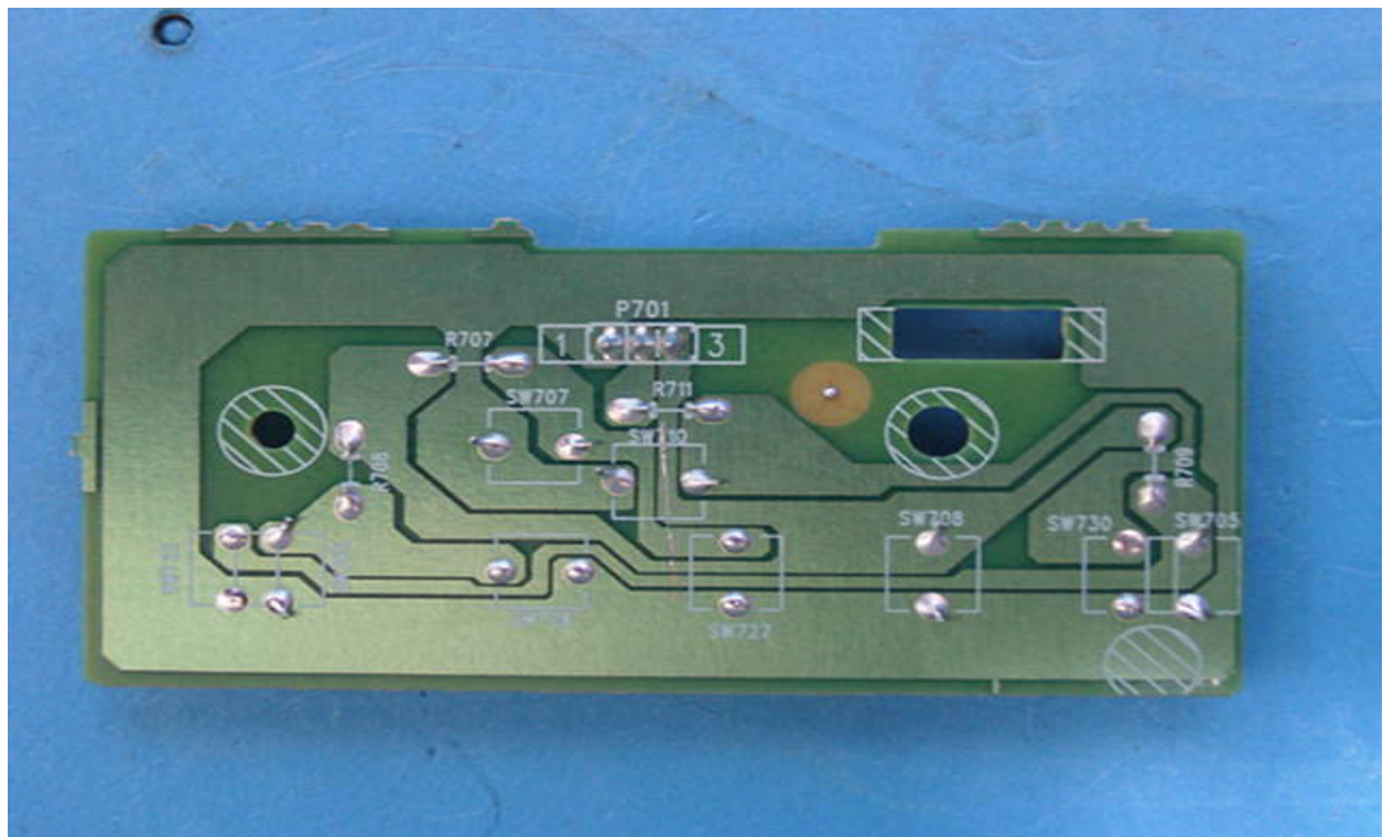
Control Panel PCB Copper View
