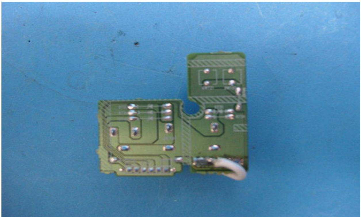
AUX front Input Panel PCB Copper View
