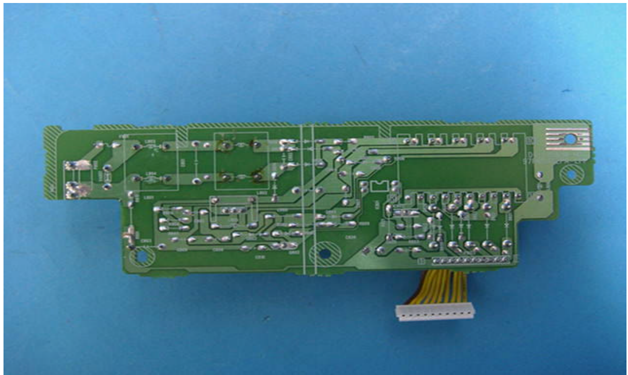
Power Board PCB Copper View
