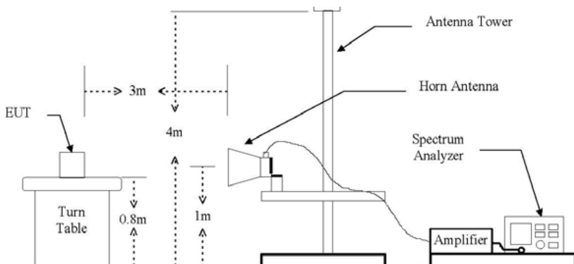
Figure 2 : Frequencies measured below 1 GHz configuration
