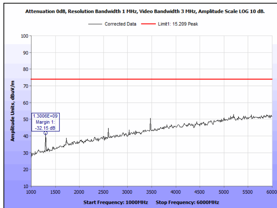
Plot 10. Field Strength of Fundamental and Harmonics, Mod2, 1 GHz – 6 GHz, Peak, No DCCF
