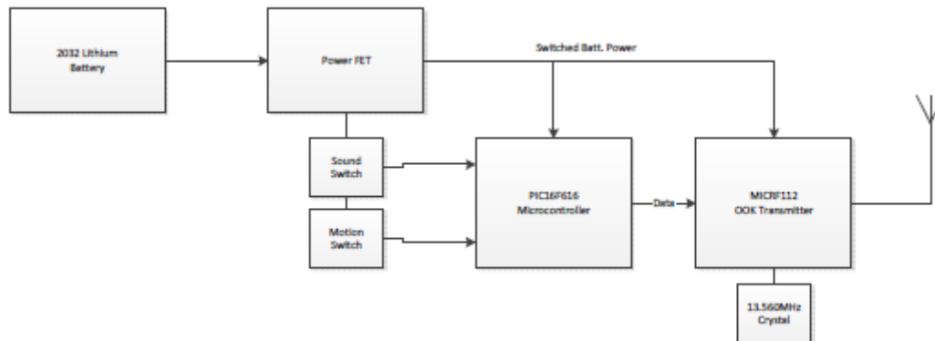
Figure 1. Block Diagram of Equipment Configuration
