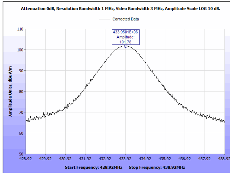
Plot 7. Field Strength of Fundamental and Harmonics, No DCCF (81.78dBuV/m with -20dB DCCF)
