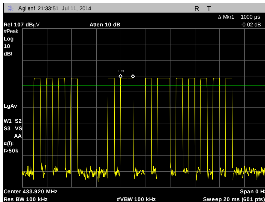
Plot 4. Periodic Operation Requirements, 433 MHz, 20ms, Long Pulse
