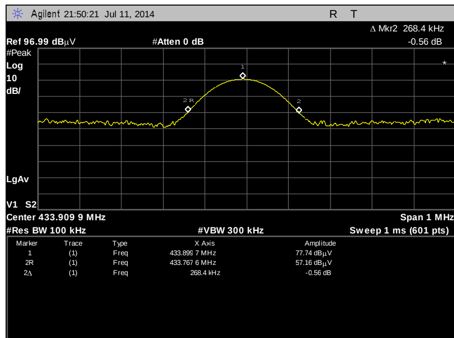
Plot 11. 20 dB Bandwidth, 433 MHz
