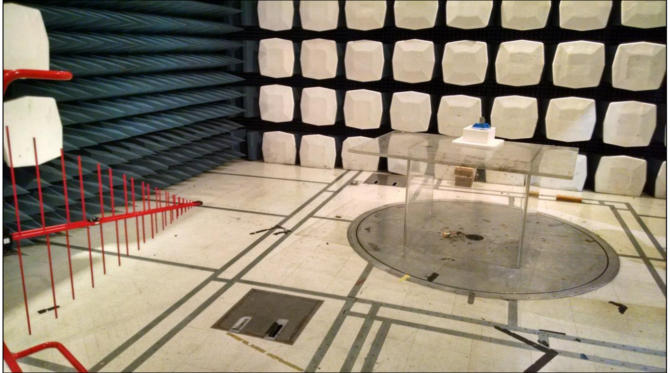
Photograph 2. Radiated Emission, Test Setup
