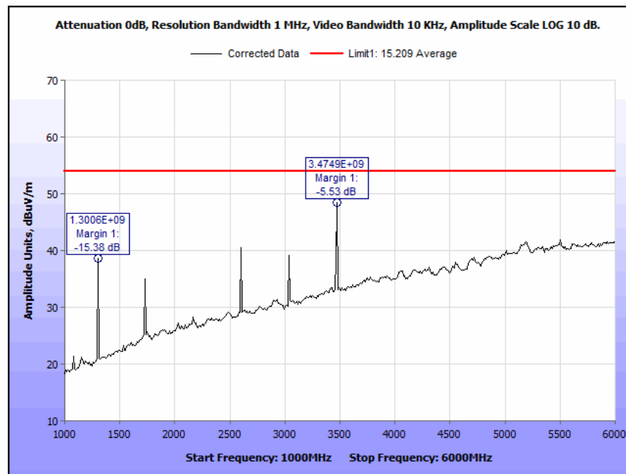
Plot 9. Field Strength of Fundamental and Harmonics, 1 GHz – 6 GHz, Average, No DCCF
