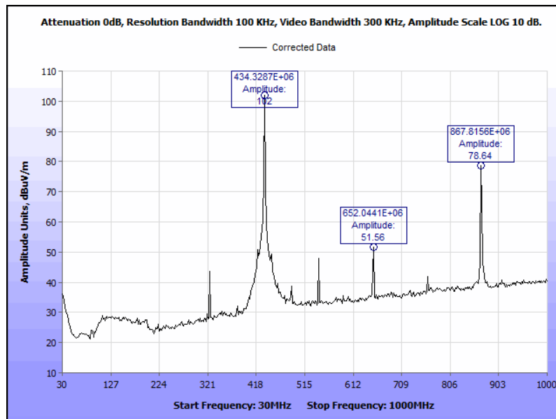
Plot 8. Field Strength of Fundamental and Harmonics, 30 MHz – 1 GHz, No DCCF
