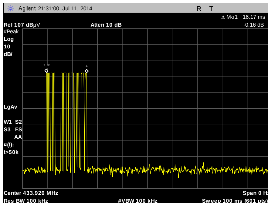
Plot 6. Periodic Operation Requirements, 433 MHz, 100ms, Period
