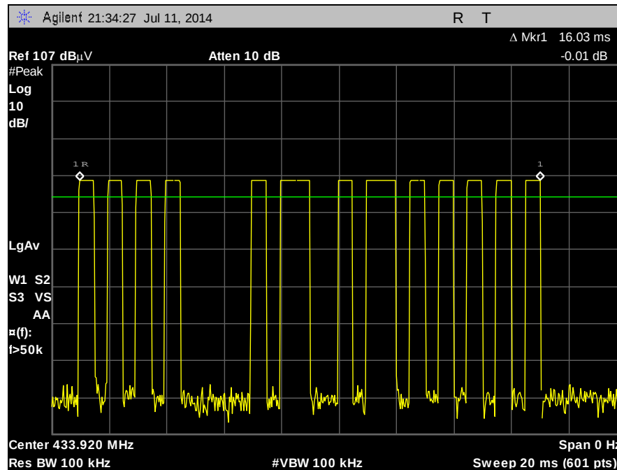
Plot 3. Periodic Operation Requirements, 433 MHz, 20ms, Period
