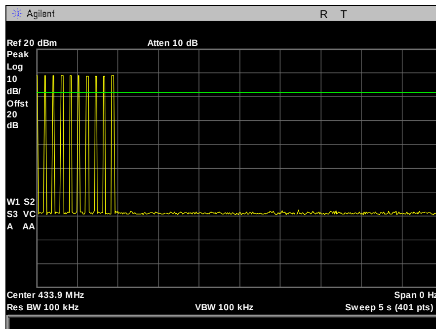
Plot 2. Periodic Operation Requirements, 5 seconds
