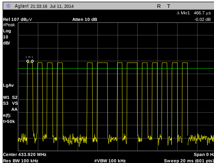
Plot 5. Periodic Operation Requirements, 433 MHz, 20ms, Short Pulse
