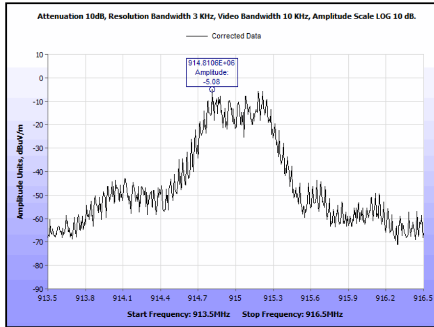
Plot 13. Peak Power Spectral Density
