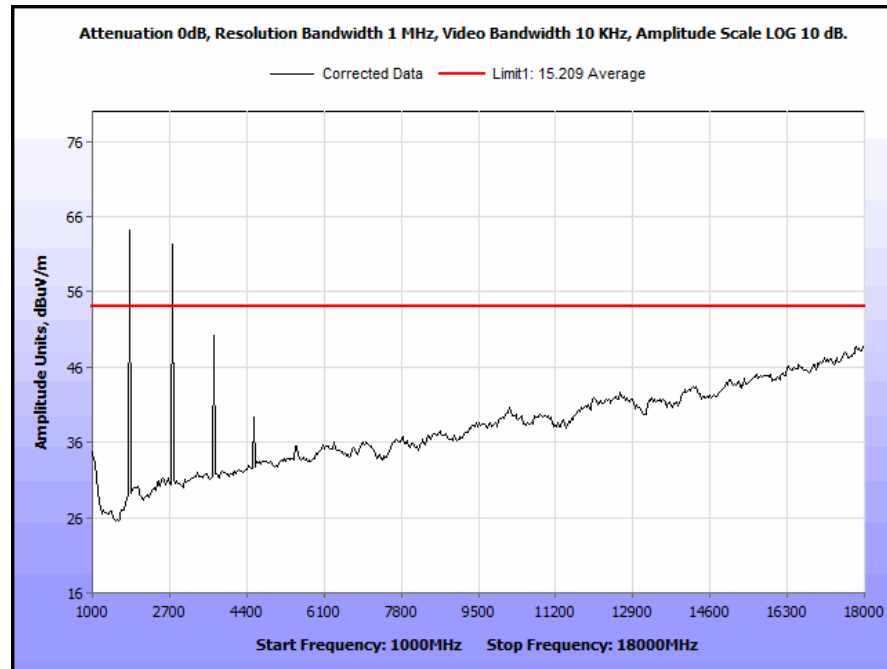
Plot 7. Radiated Spurious Emissions, Above 1 GHz, 10 kHz, VBW, Average
