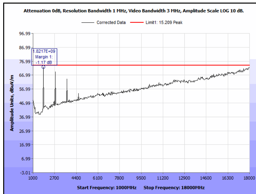
Plot 8. Radiated Spurious Emissions, Above 1 GHz, Peak
