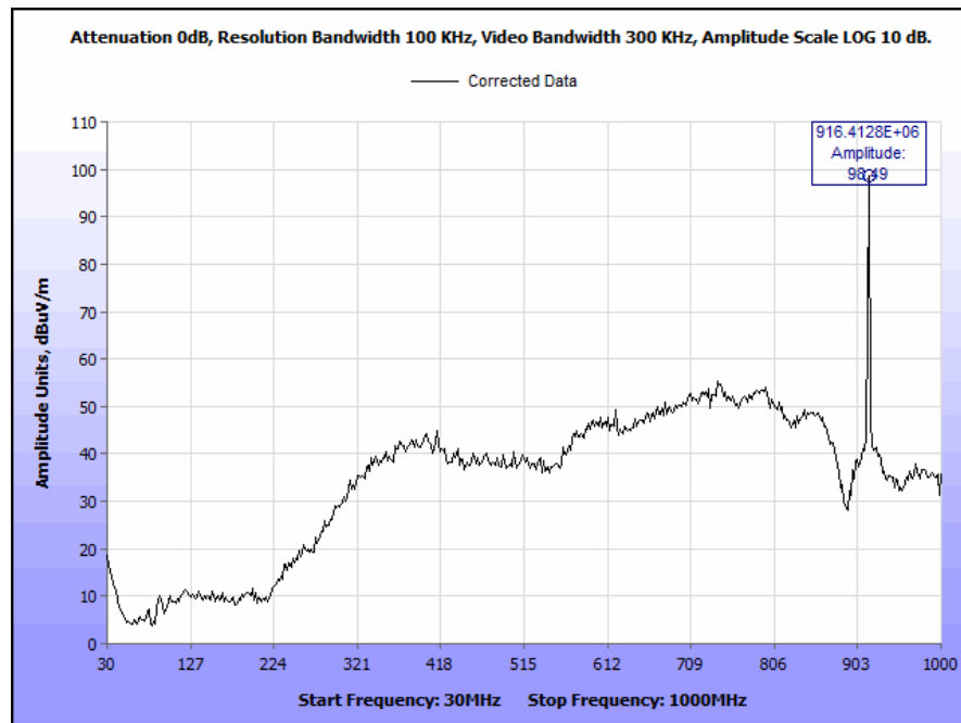
Plot 11. Conducted Spurious Emissions, 30 MHz – 1 GHz with Markers
