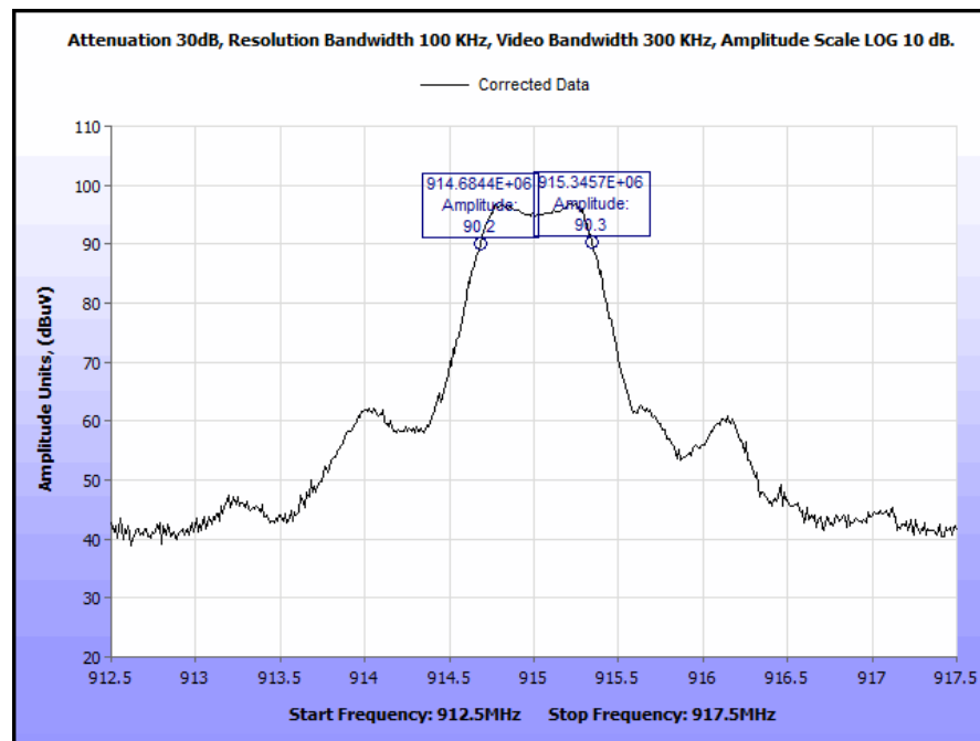
Plot 1. 6 dB Occupied Bandwidth
