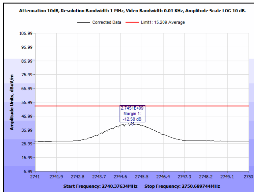
Plot 6. Radiated Spurious Emissions, 2.745 GHz (Zoomed), Average
