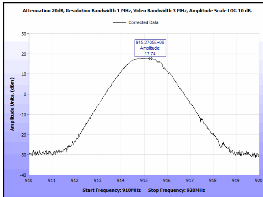
Plot 2. Peak Power Output
