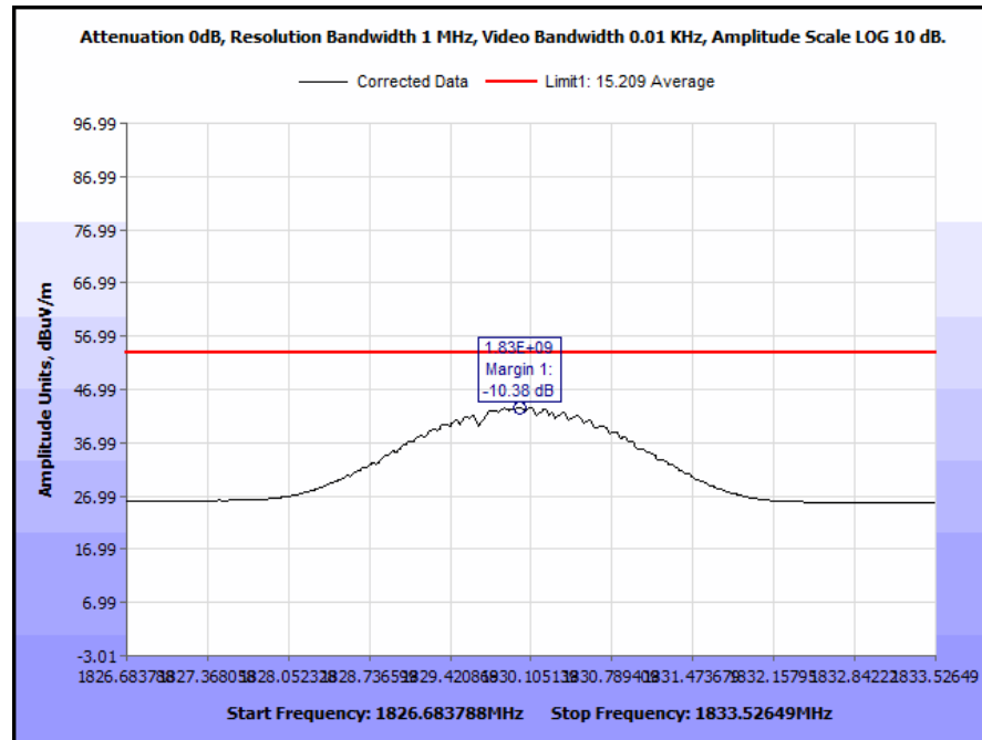
Plot 5. Radiated Spurious Emissions, 1.83 GHz (Zoomed), Average
