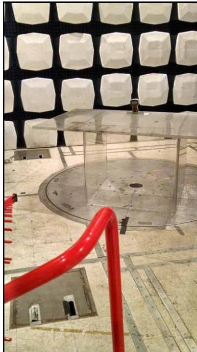
Photograph 1. Radiated Spurious Emissions, Test Setup, 30 MHz – 1 GHz
