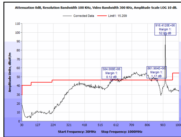
Plot 3. Radiated Spurious Emissions, 30 MHz – 1 GHz with Markers
