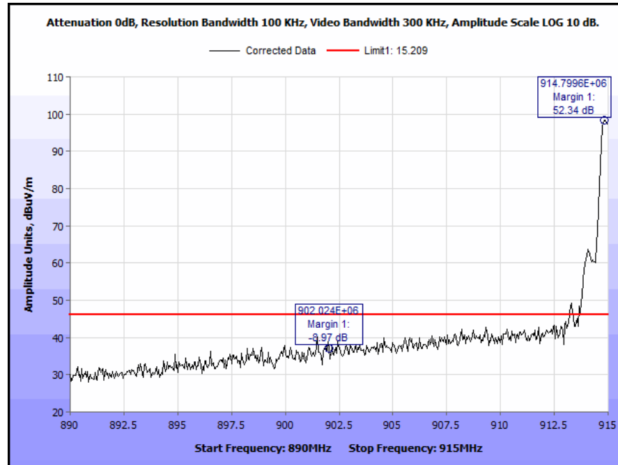
Plot 9. Radiated Restricted Band Edge, Low
