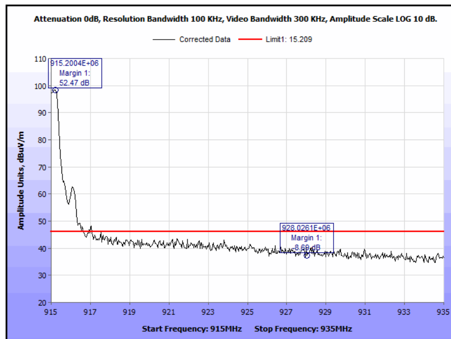
Plot 10. Radiated Restricted Band Edge, High
