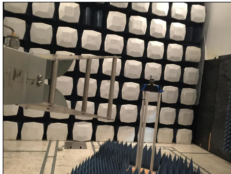
Photograph 2. Radiated Spurious Emissions, Test Setup, Above 1 GHz
