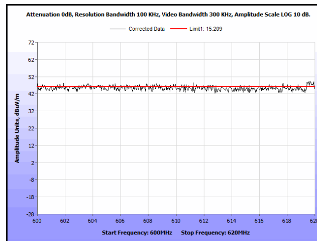
Plot 4. Radiated Spurious Emissions, 600 MHz – 620 MHz
