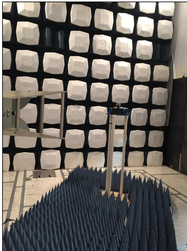
Photograph 2. Radiated Spurious Emissions, Test Setup, Above 1 GHz
