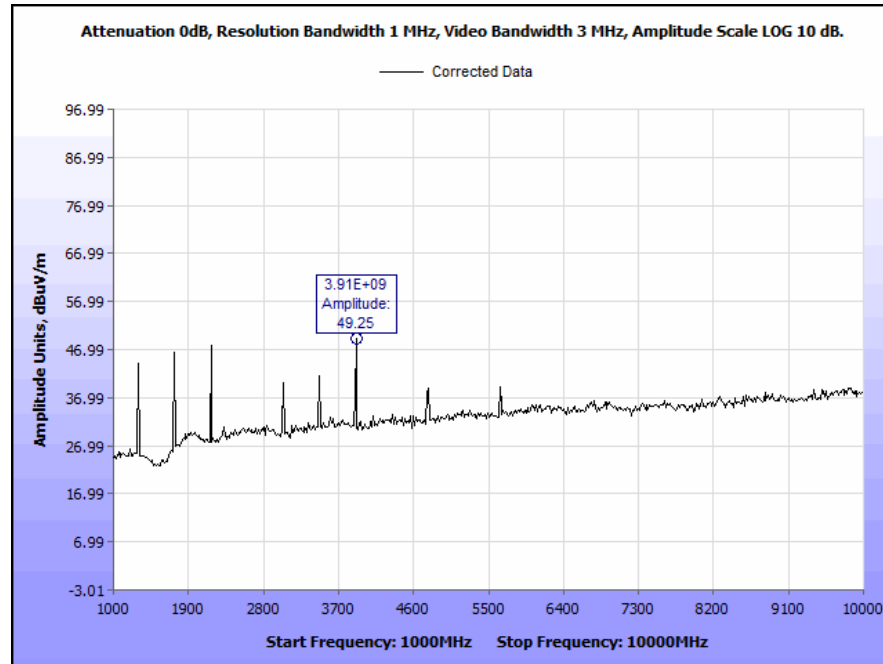
Plot 7. Radiated Spurious Emissions, Harmonics with Restricted Band, Above 1 GHz (Peak under Average Limit)
