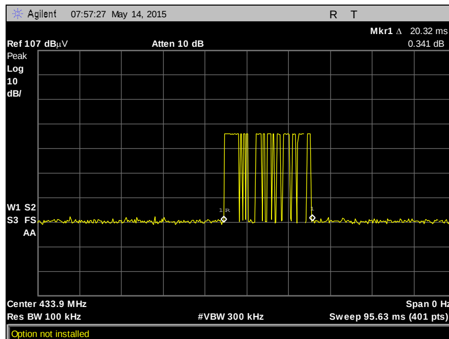
Plot 3. On Time
