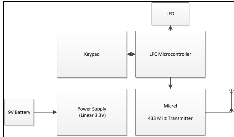
Figure 1. Block Diagram of Equipment Configuration
