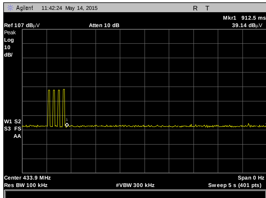
Plot 1. Periodic Operation
