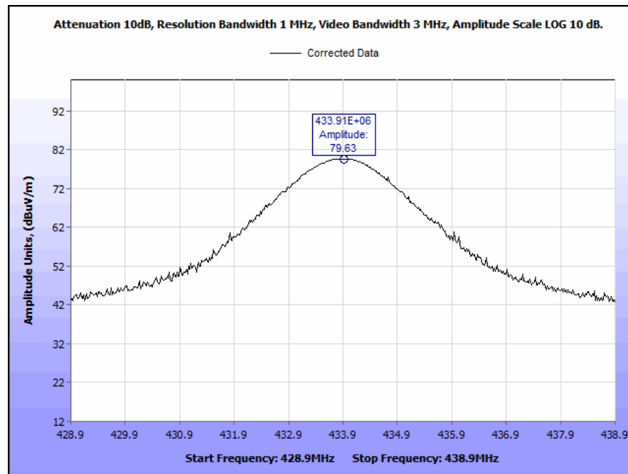
Plot 5. Fundamental Field Strength (corrected for duty cycle)
