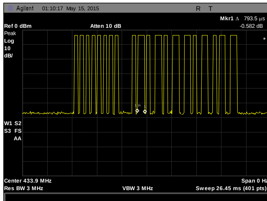
Plot 5. On Time, Zoomed (Wide Pulses Time)
