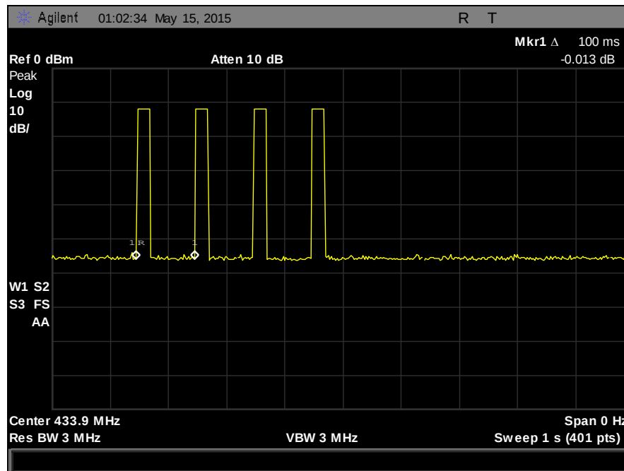
Plot 2. Transmission Period in 100 ms
