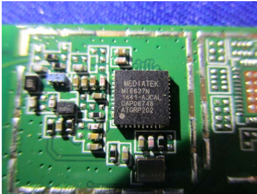
EUT –WiFi&BT&GPS RF Chip View
