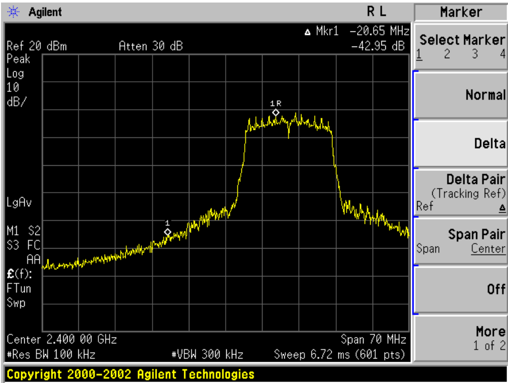
802.11g- CH1
