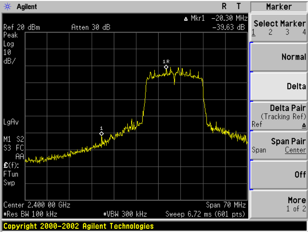
802.11n-CH1
