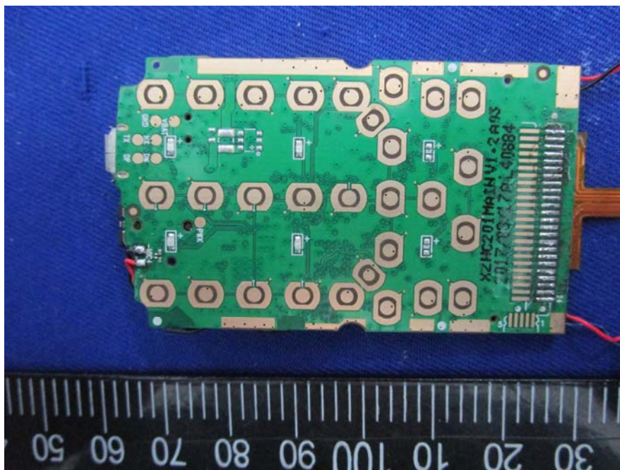
EUT –Mainboard Unshiled Bottom View
