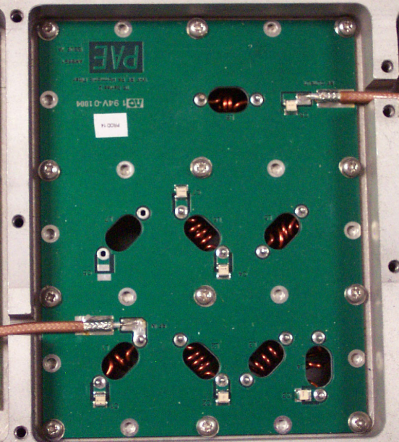
Filter -Part of PA assembly
