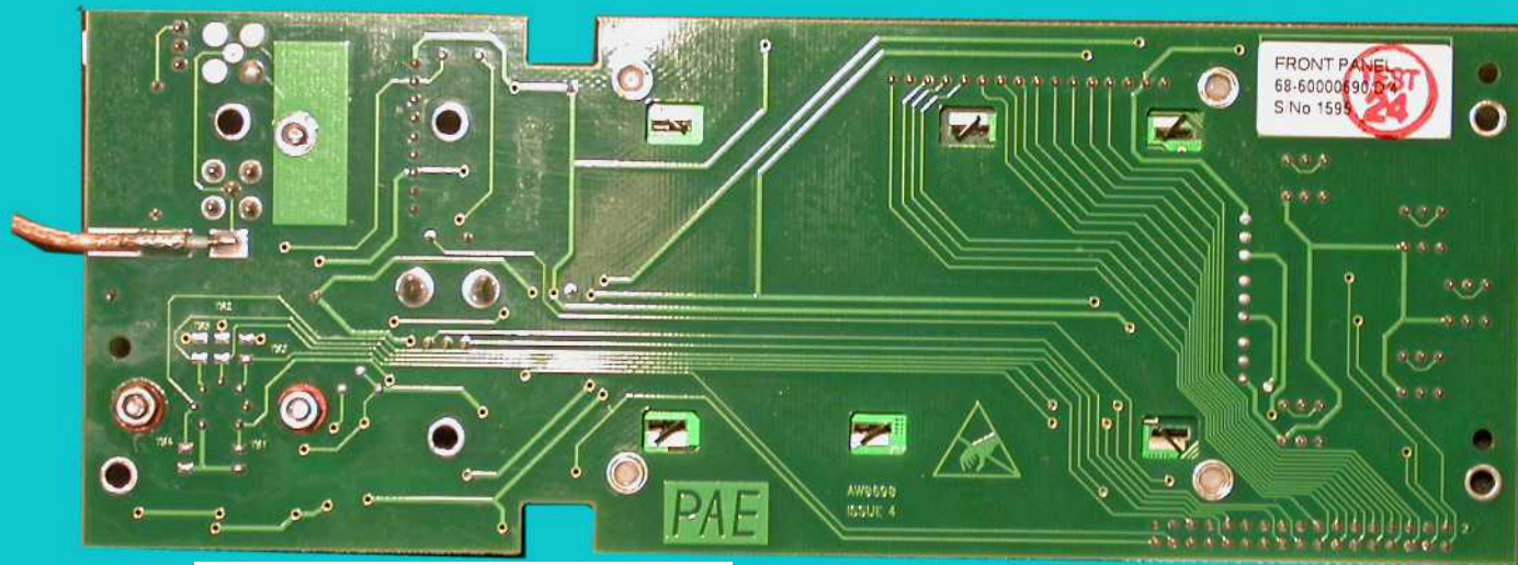
Front panel 68-60000690
