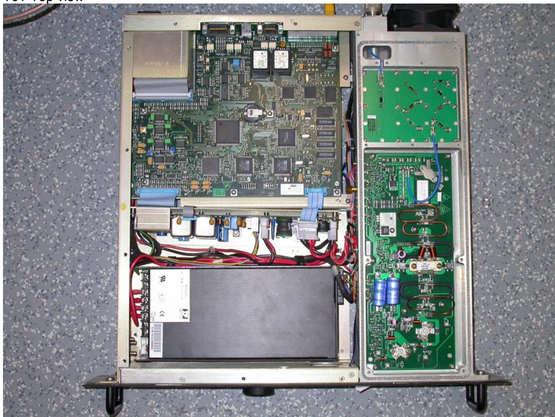
T6T Top view
