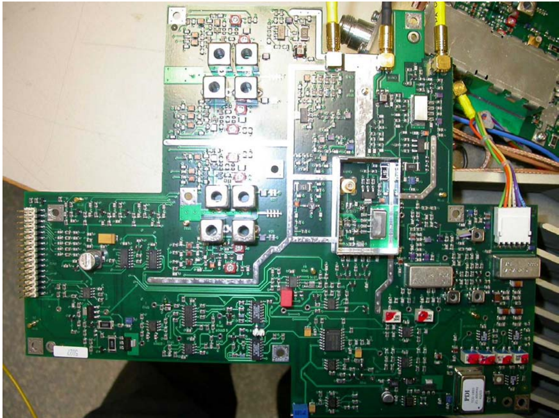
T6TR PA Control module
