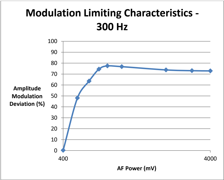
Figure 27 - Modulation Limiting Capability - 300 Hz AF
