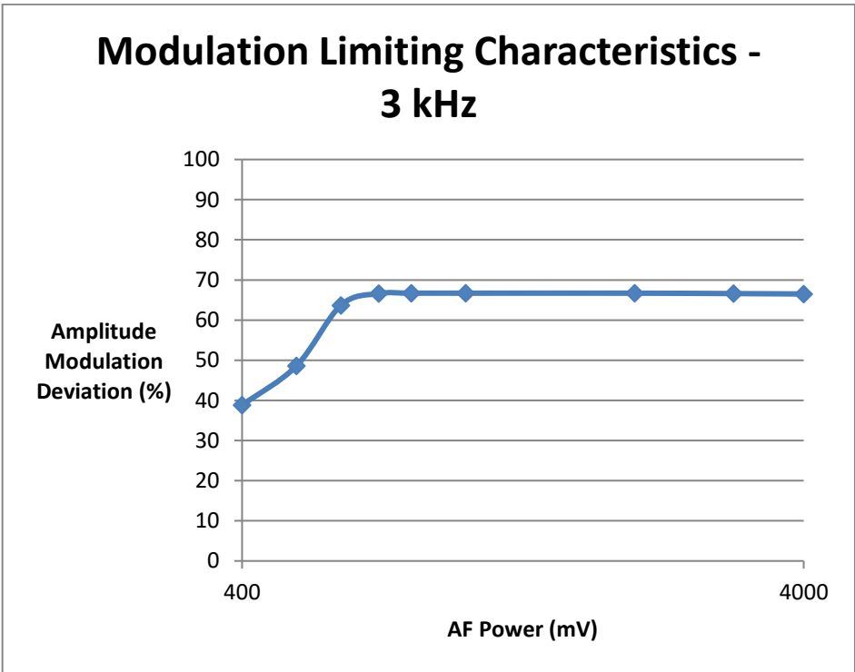
Figure 29 - Modulation Limiting Capability - 3 kHz AF
