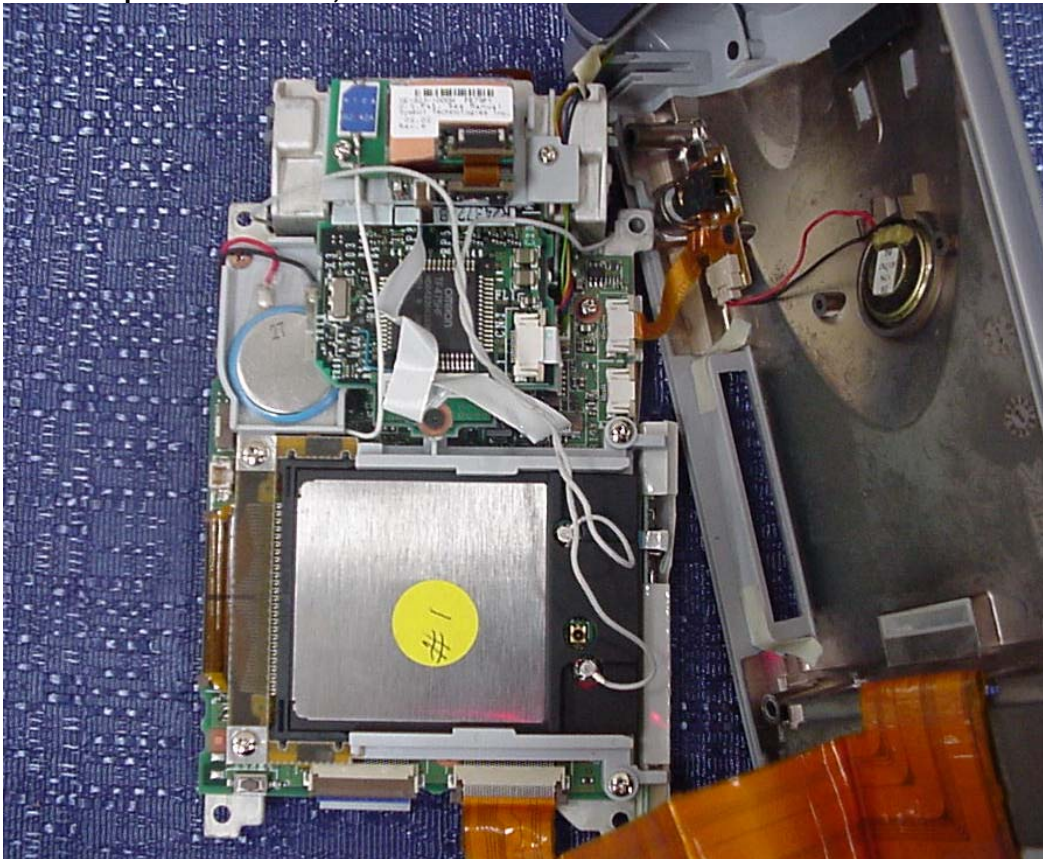
Test Sample B-PAD/ iPad, Model CA06178-A3xx – internal view
