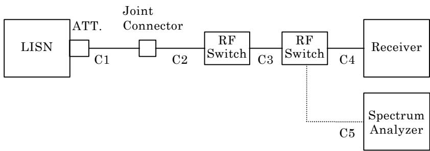
Schema for the conducted measurement
