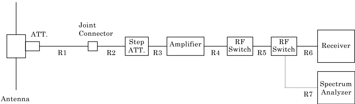
Schema for the radiated measurement
