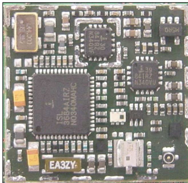
Front View of WLAN module without shielding
