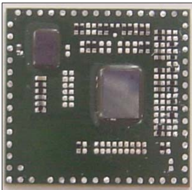
Rear View of WLAN module with shielding
