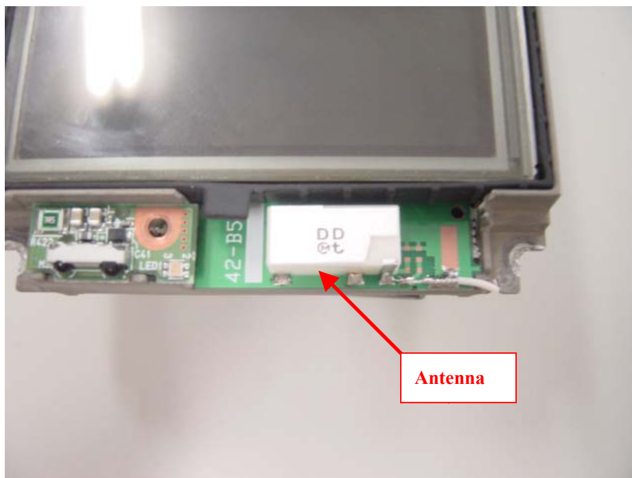
WLAN Antenna
