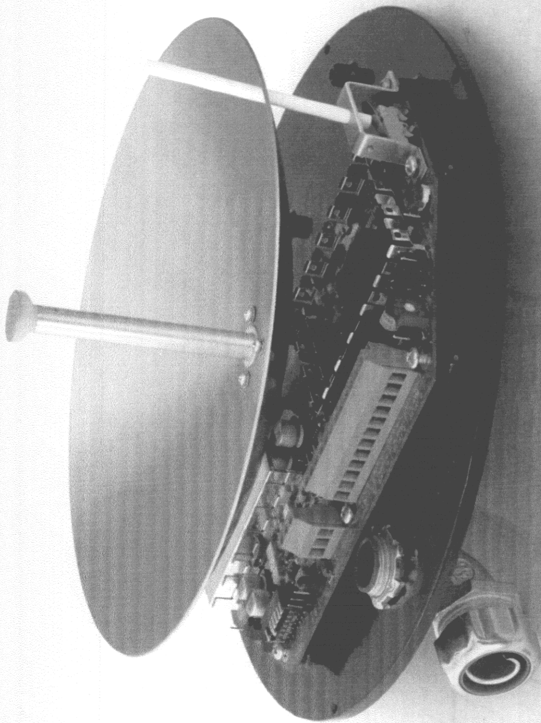
FIGURE 1 MODEL 316R RECEIVER WITHOUT RADOME
