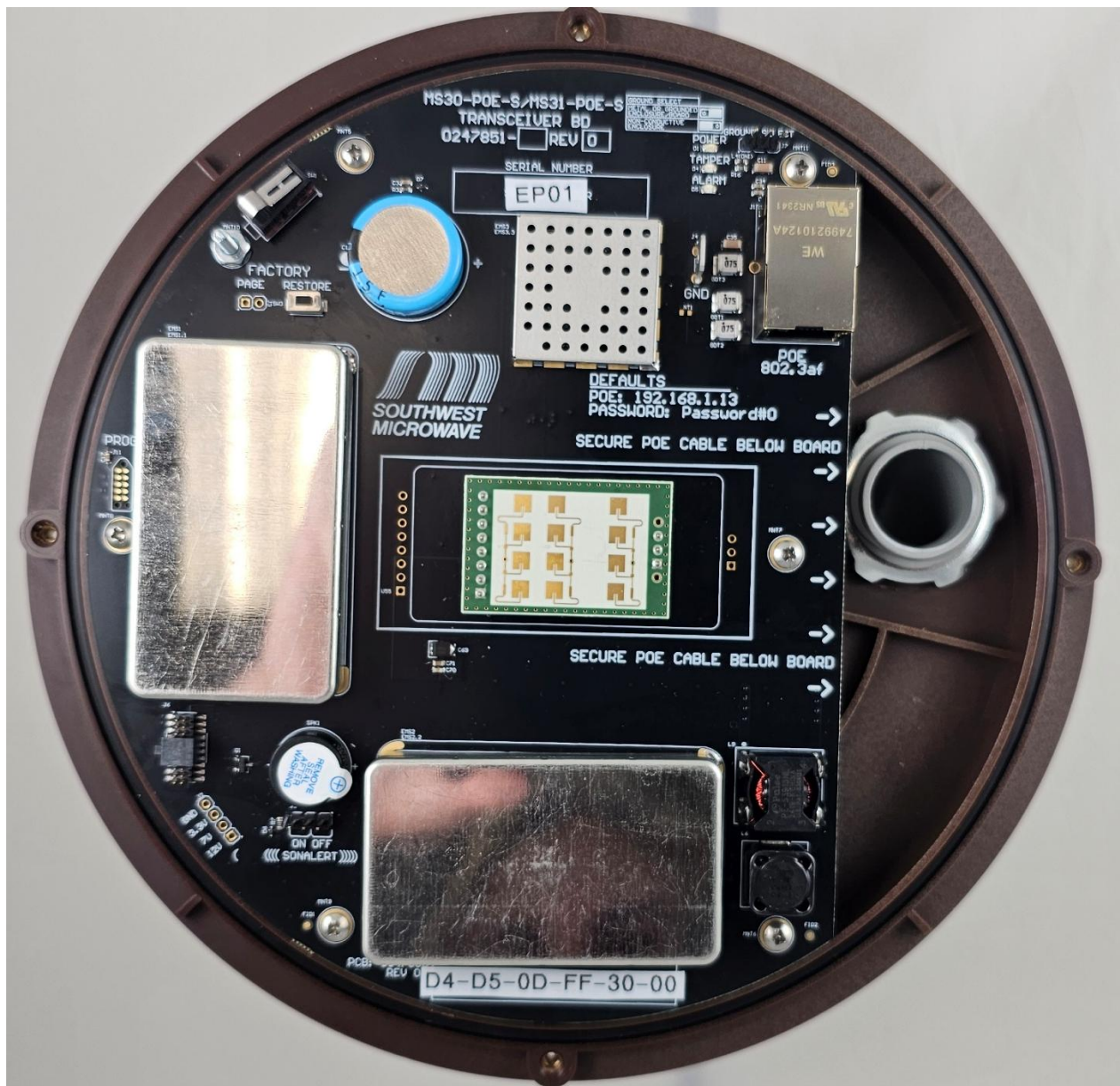
Internal with Shield Cans
