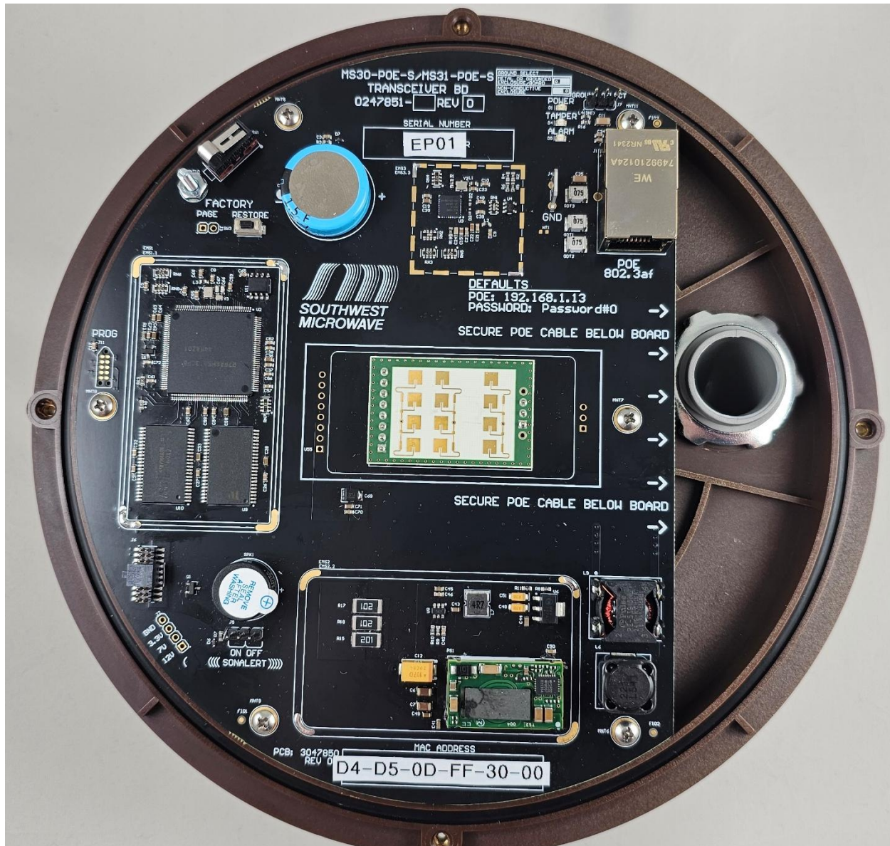
Internal Without Shield Cans
