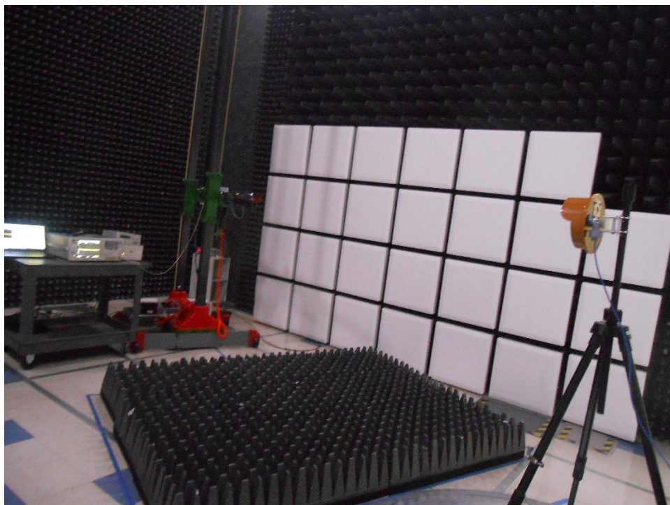
Radiated Emissions Test set up 40 -50 GHz (2)
