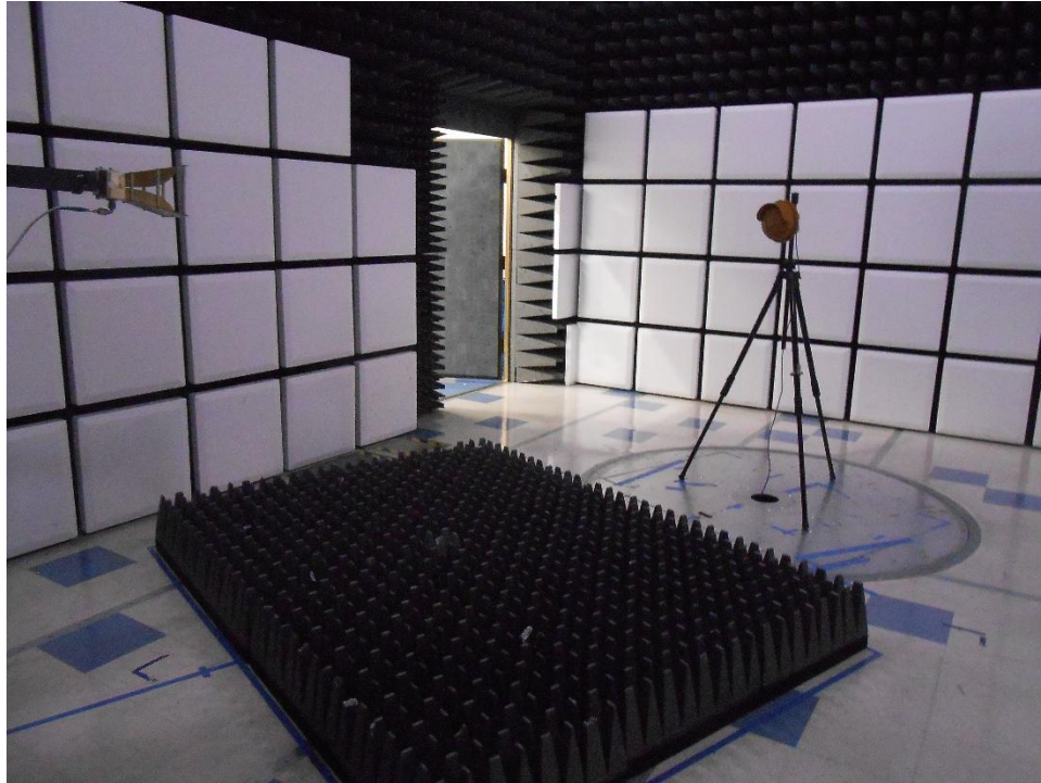
Radiated Emissions Test set up 1 – 18 GHz (2)
