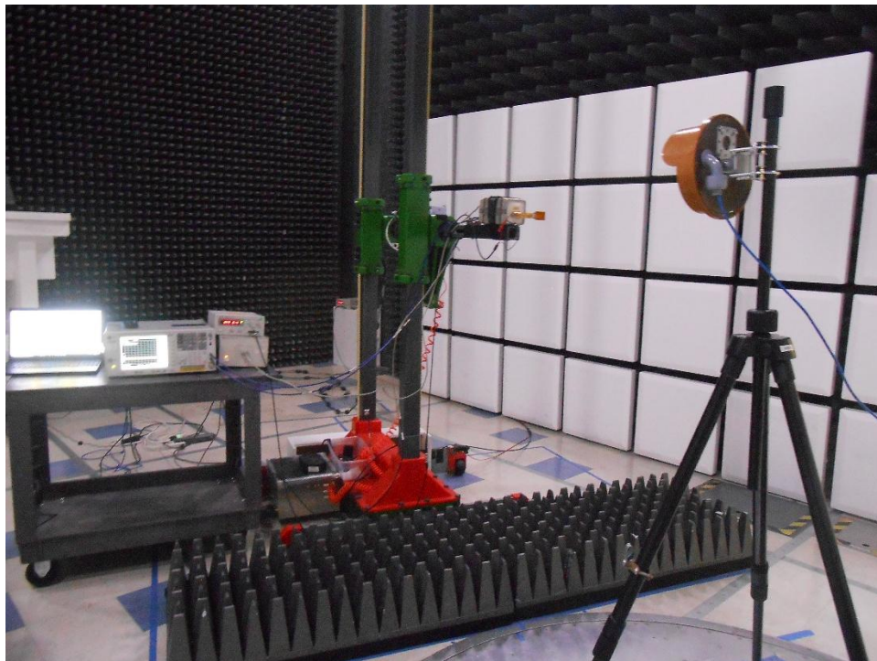
Radiated Emissions Test set up 50 – 75 GHz (2)
