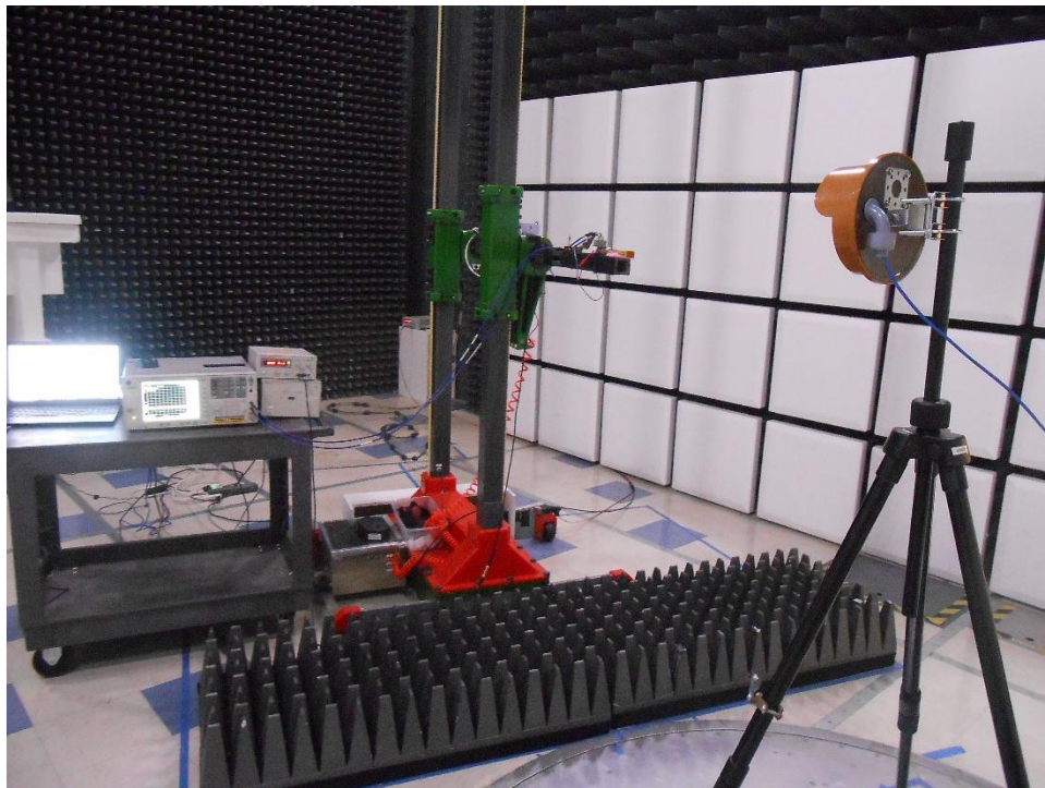
Radiated Emissions Test set up 30 - 1000 MHz (2)
