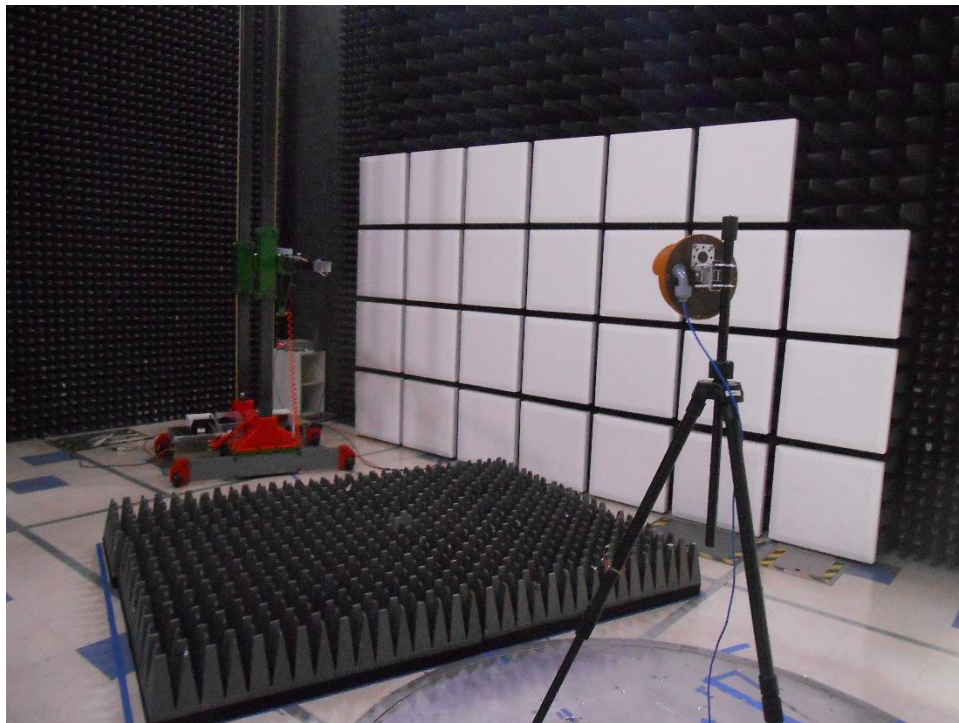
Radiated Emissions Test set up 18 – 40 GHz (2)
