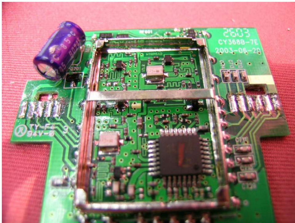
Base Oscillator PCB comp side (View 4)
