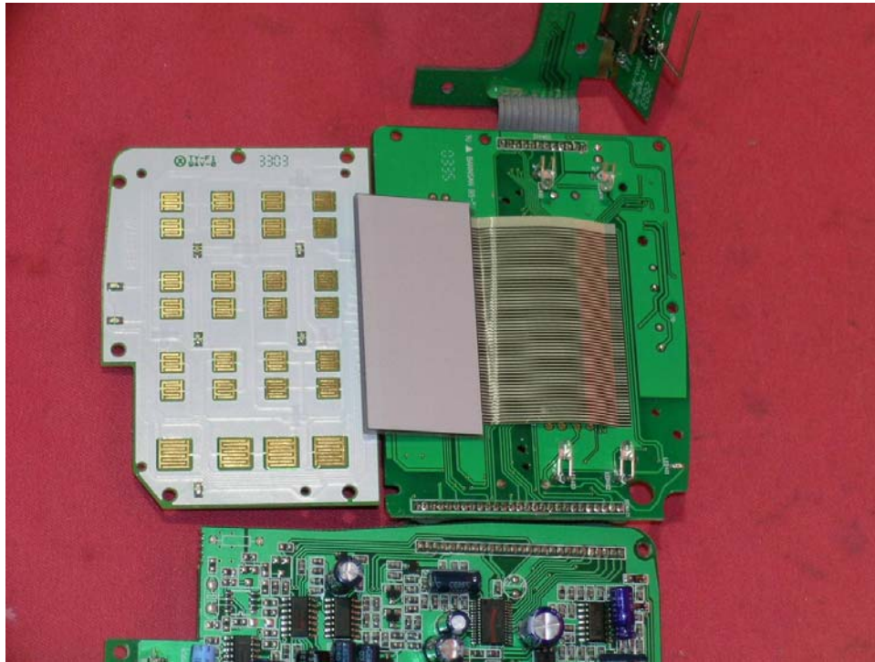
Base LCD Display and Keypad front side (view 2)
