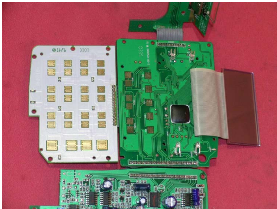
Base LCD Display and Keypad front side (view 1)
