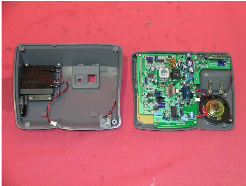
Base assembly
