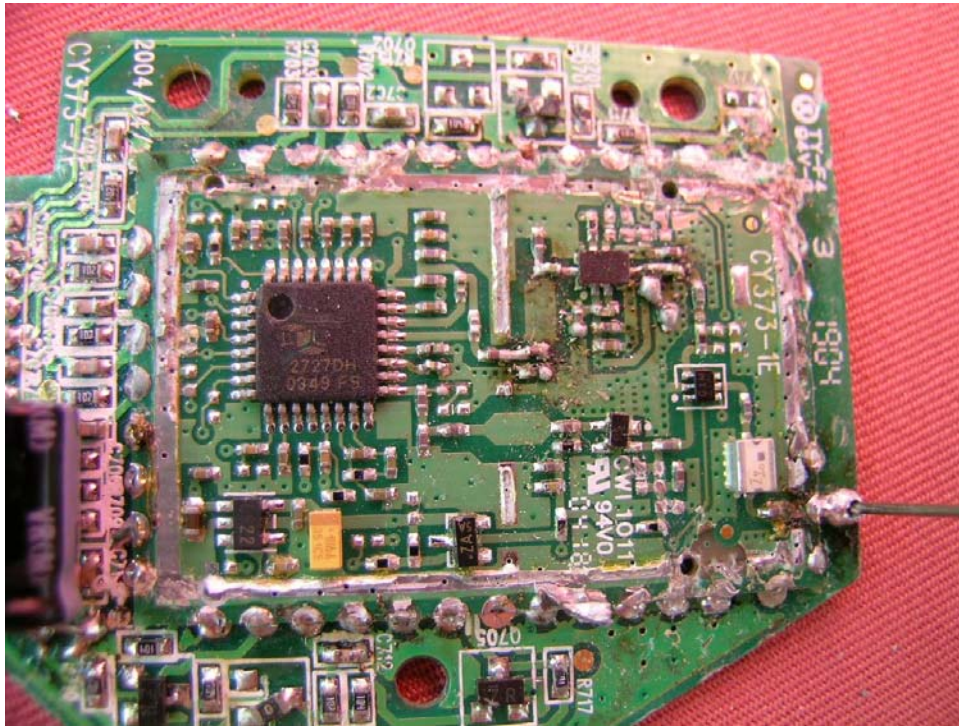
Base Oscillator PCB comp side (RF module 1) - View 2
