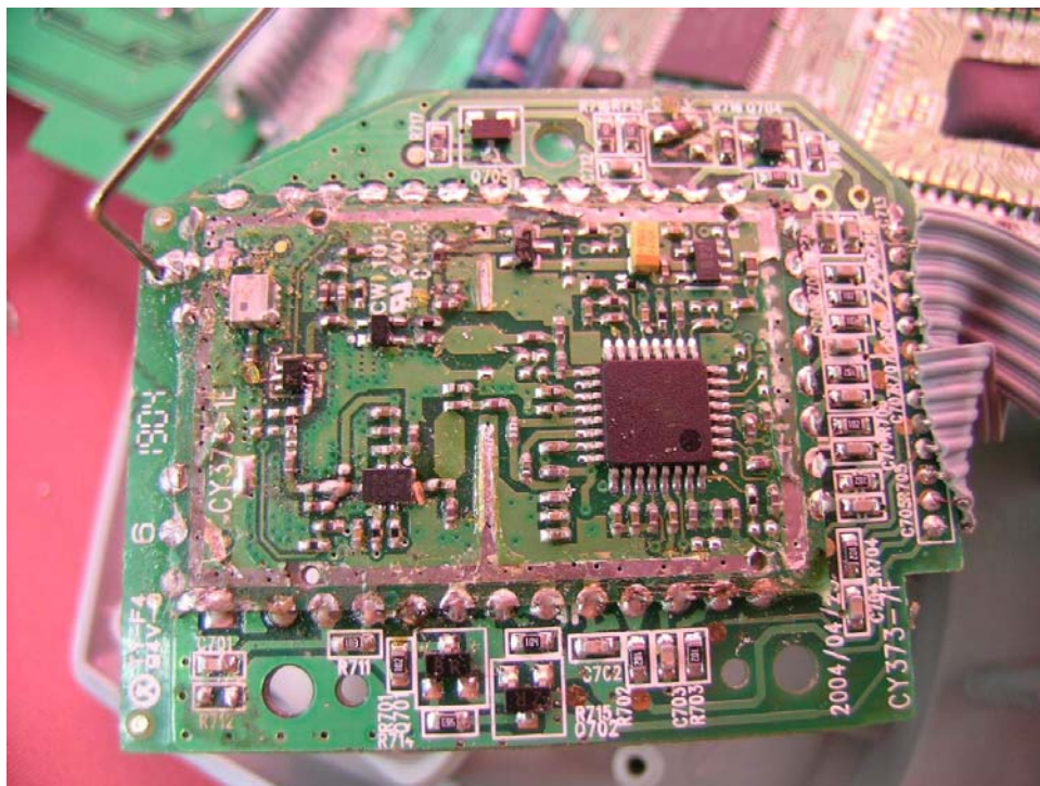
Base Oscillator PCB comp side (RF module 2) - View 2
