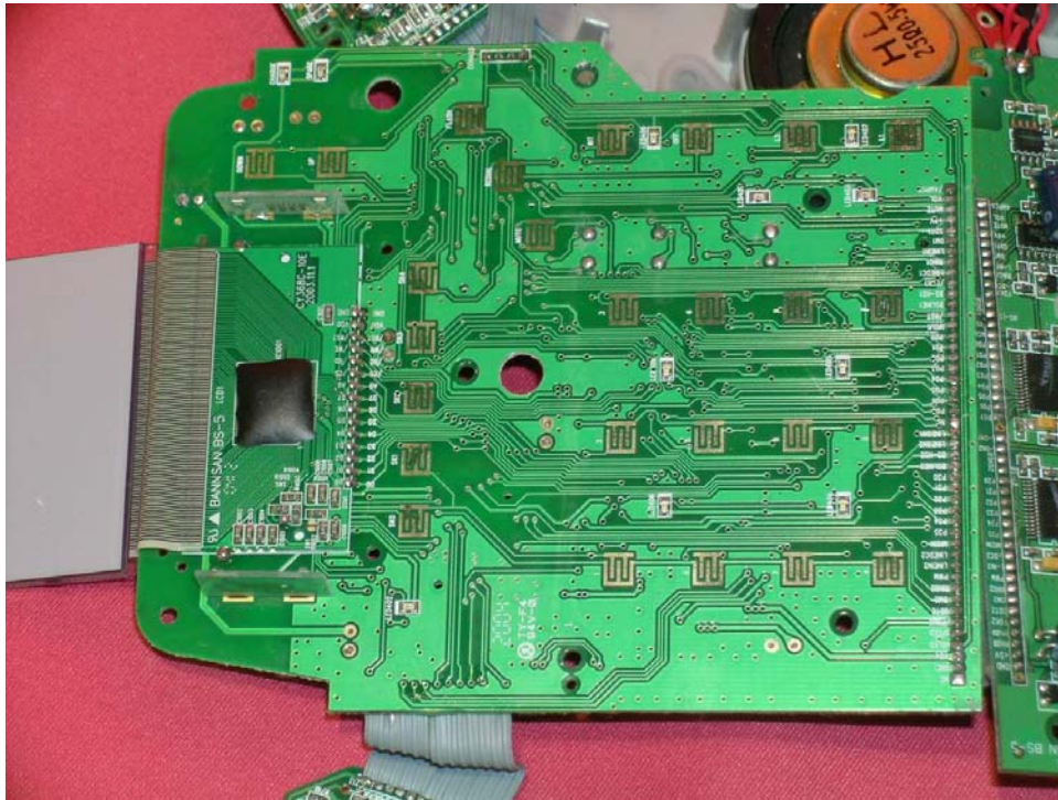
Base Keypad and LCD Display solder side (View 1)
