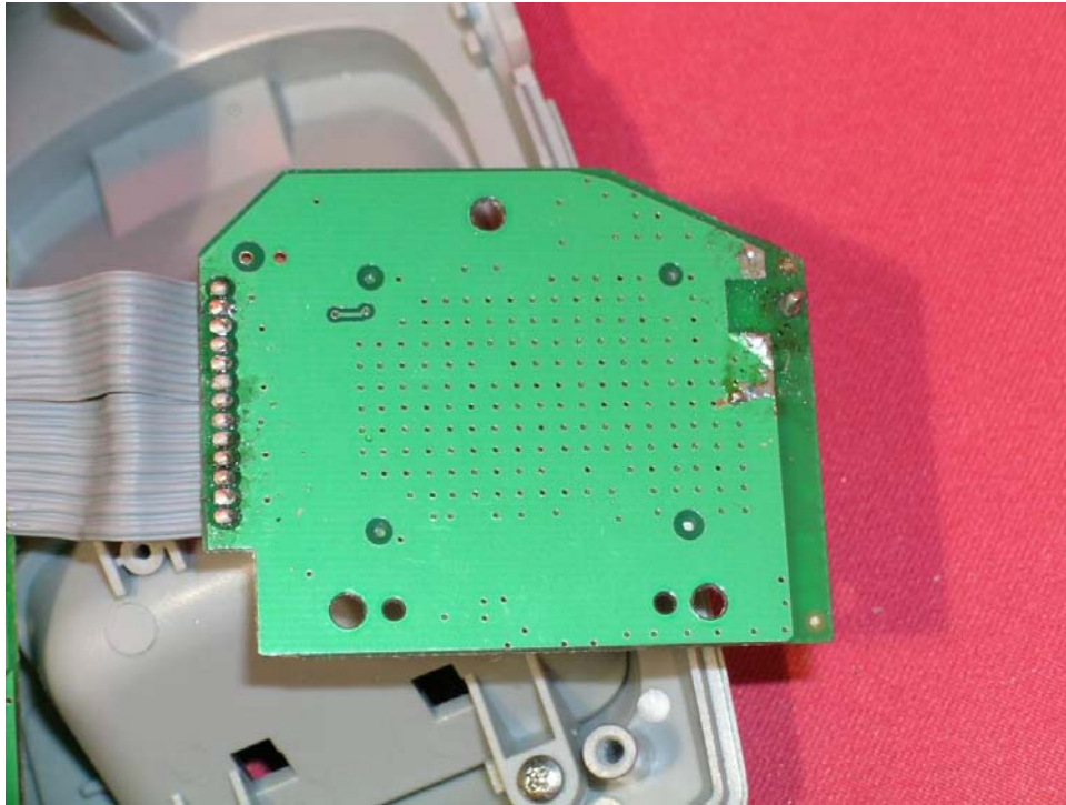
Base Oscillator PCB solder side (RF module 2)
