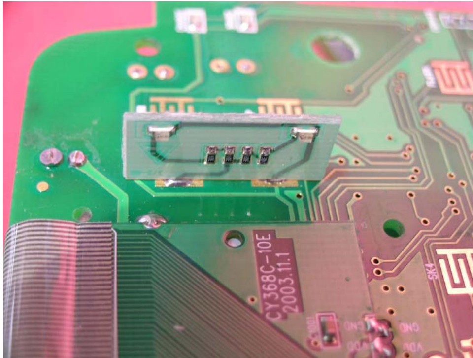
Base Keypad and LCD Display solder side (View 3)
