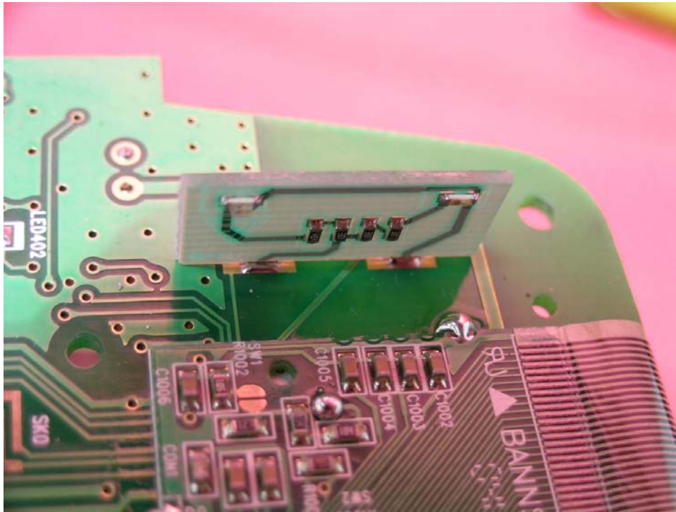
Base Keypad and LCD Display solder side (View 5)
