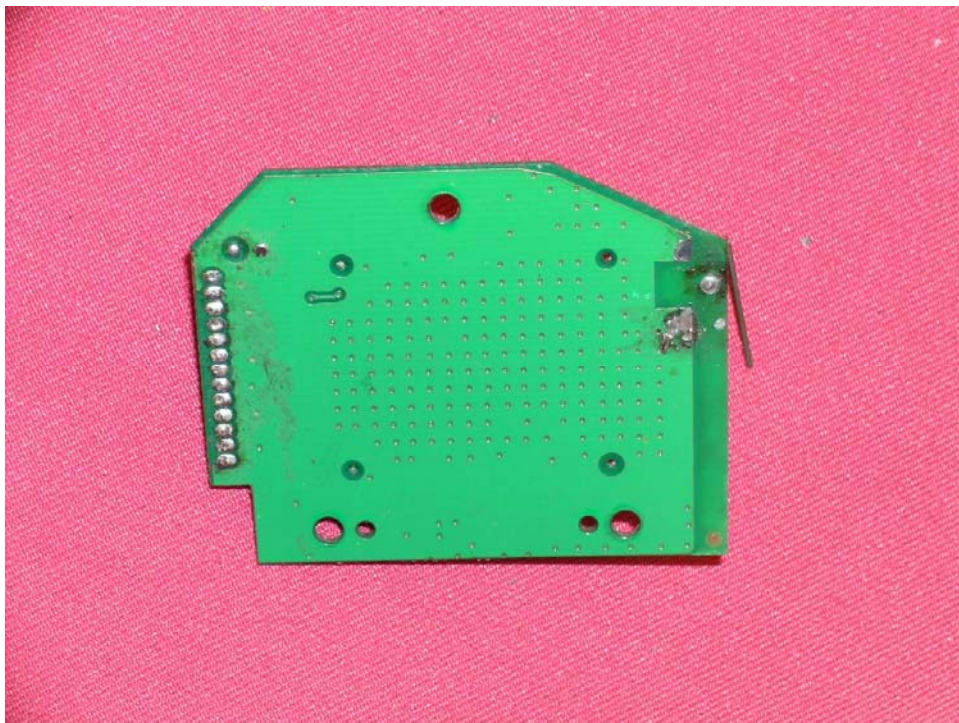
Base Oscillator PCB solder side (RF module 1)
