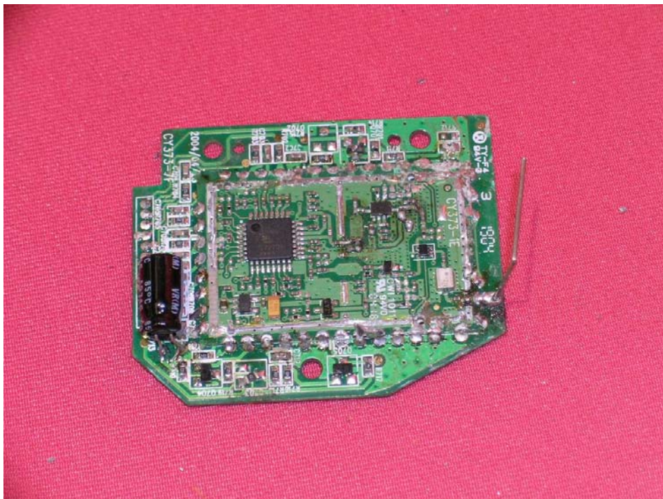
Base Oscillator PCB comp side (RF module 1) - View 1
