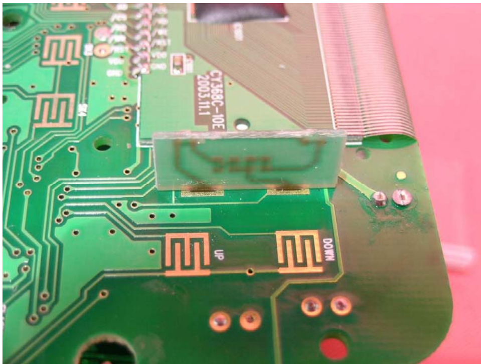
Base Keypad and LCD Display solder side (View 2)
