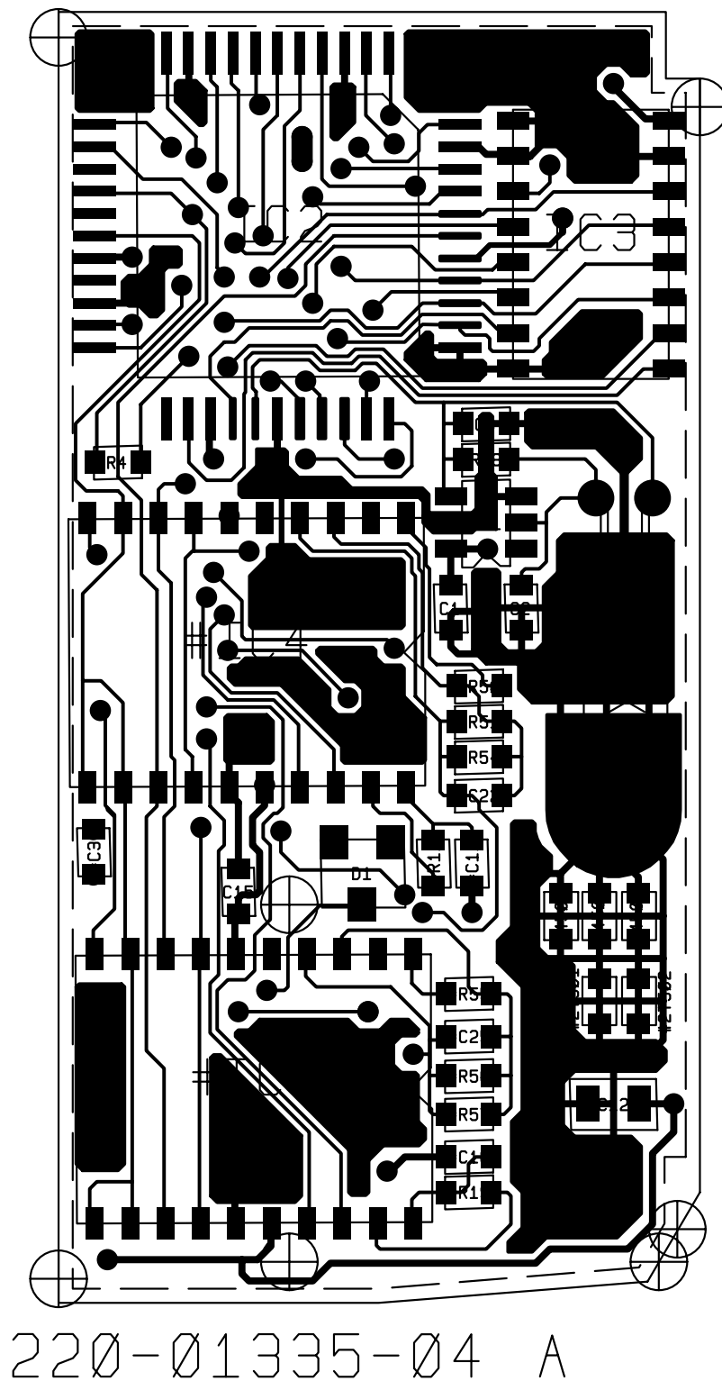
T2000-A450X PCB (IPN 220-01335-04) - Top Side
