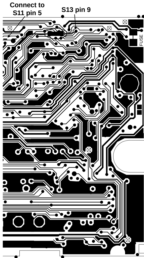
T2010 & T2015 Logic PCB - Bottom Side
