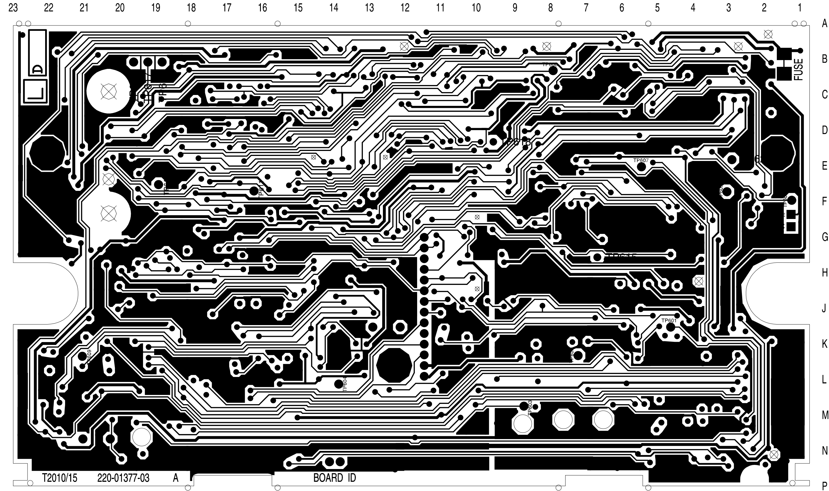
T2010 & T2015 HC05 Logic PCB Bottom Side Layout IPN 220-01377-03
