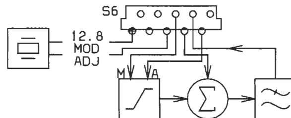
Figure 2.1 T2000 TCXO/TX Audio PCB Block Diagram
