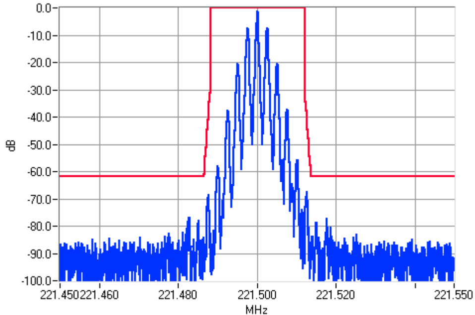
Analogue Modulation 221.5000MHz Mask Fx5 5W Pass
