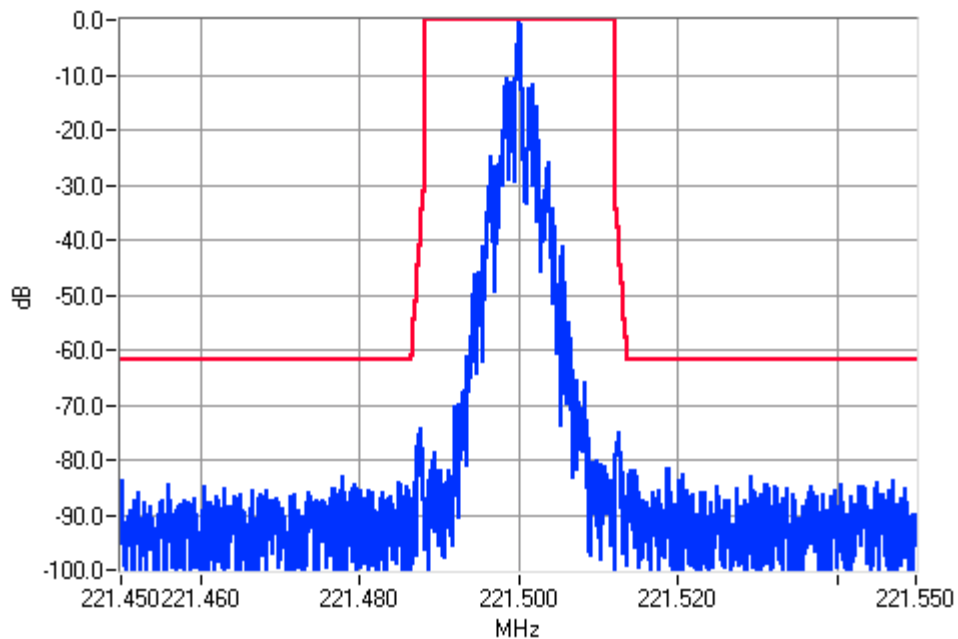
Digital Modulation 221.5000MHz Mask Fx5 5W Pass
