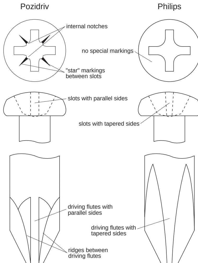
Figure 3.2 Screwdriver Identification
