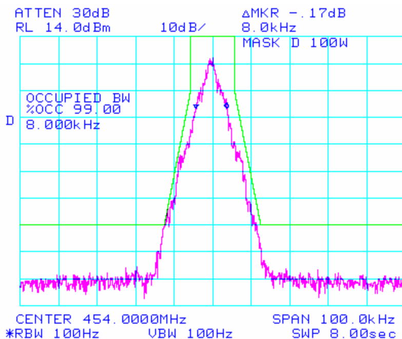
Plot 3a: MASK D, 8K00F1D, OUTPUT POWER: 25 Watts
