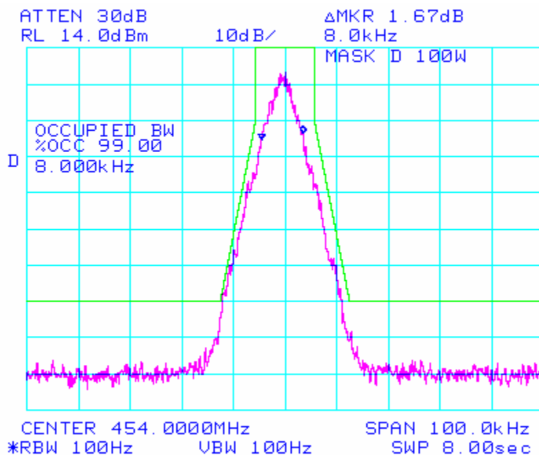
Plot 2a: MASK D, 8K00F1D, OUTPUT POWER: 25 Watts
