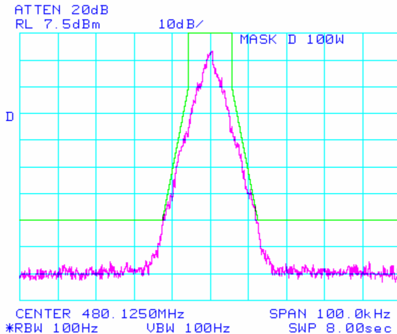
Plot 3b: MASK D, 8K17F1D, OUTPUT POWER: 5 Watts
