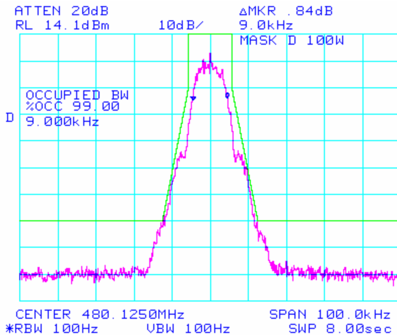
Plot 1a: MASK D, 9K00F1D, OUTPUT POWER: 25 Watts
