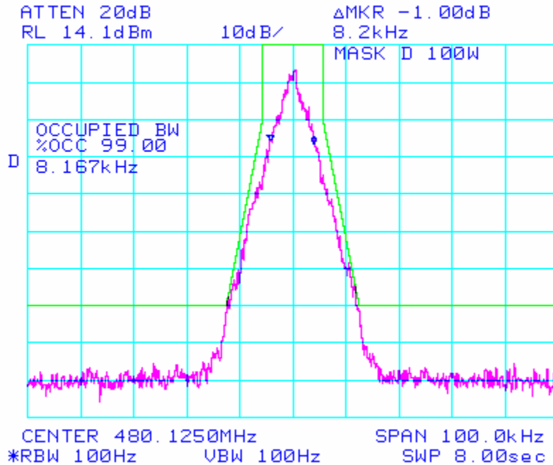
Plot 3a: MASK D, 8K17F1D, OUTPUT POWER: 25 Watts
