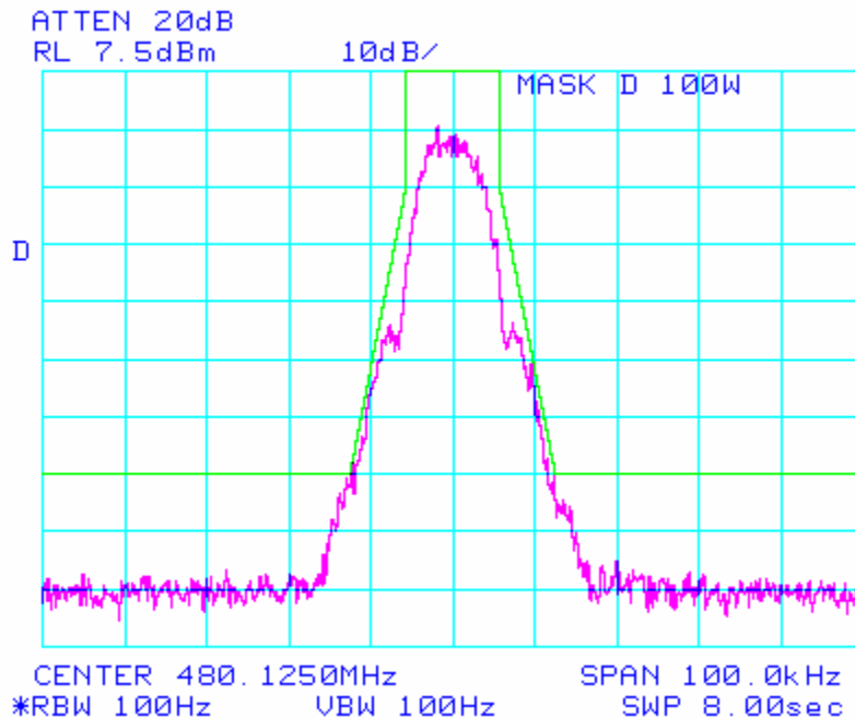
Plot 1b: MASK D, 9K00F1D, OUTPUT POWER: 5 Watts
